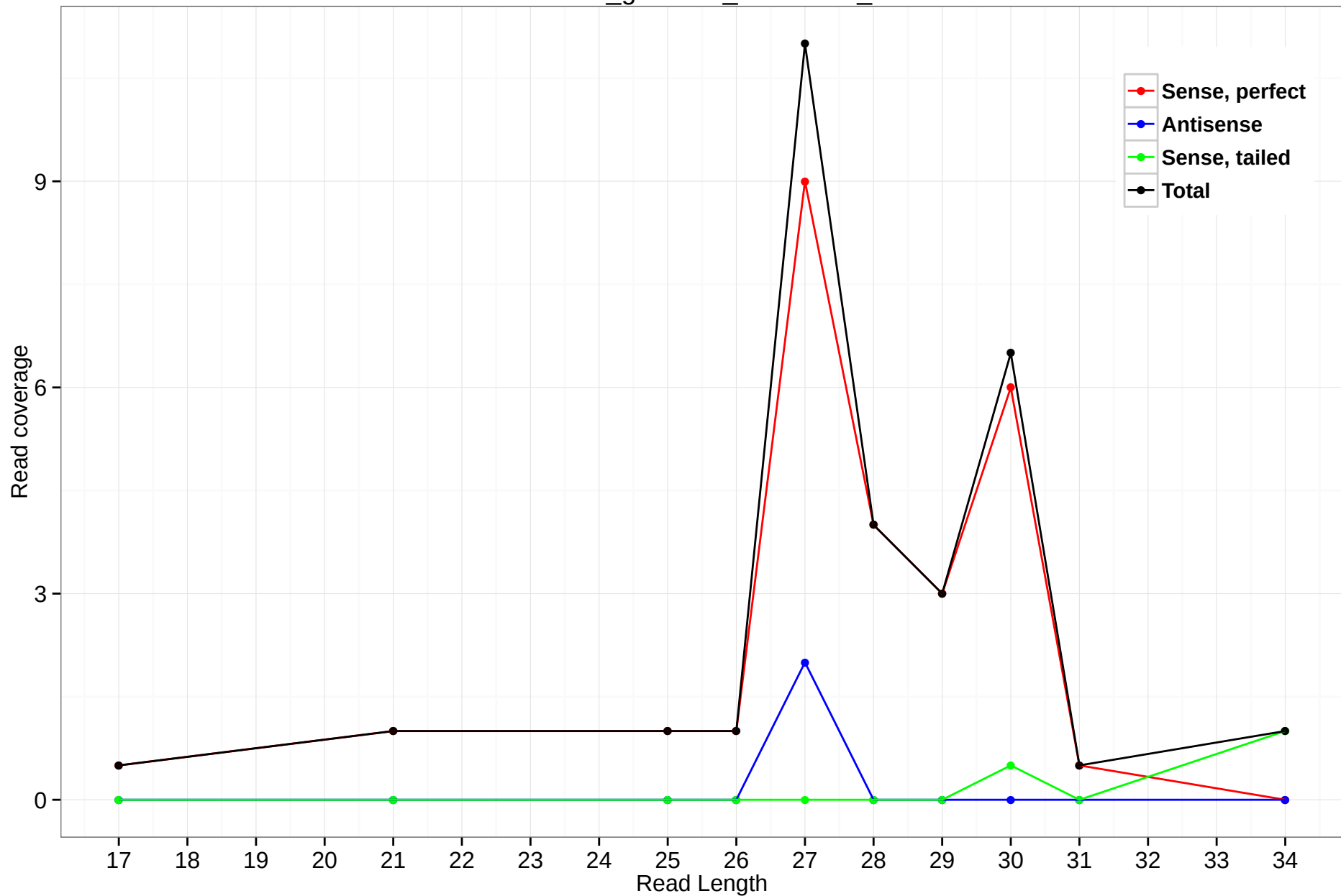
rheMac3_genscan_chr15.196_19
