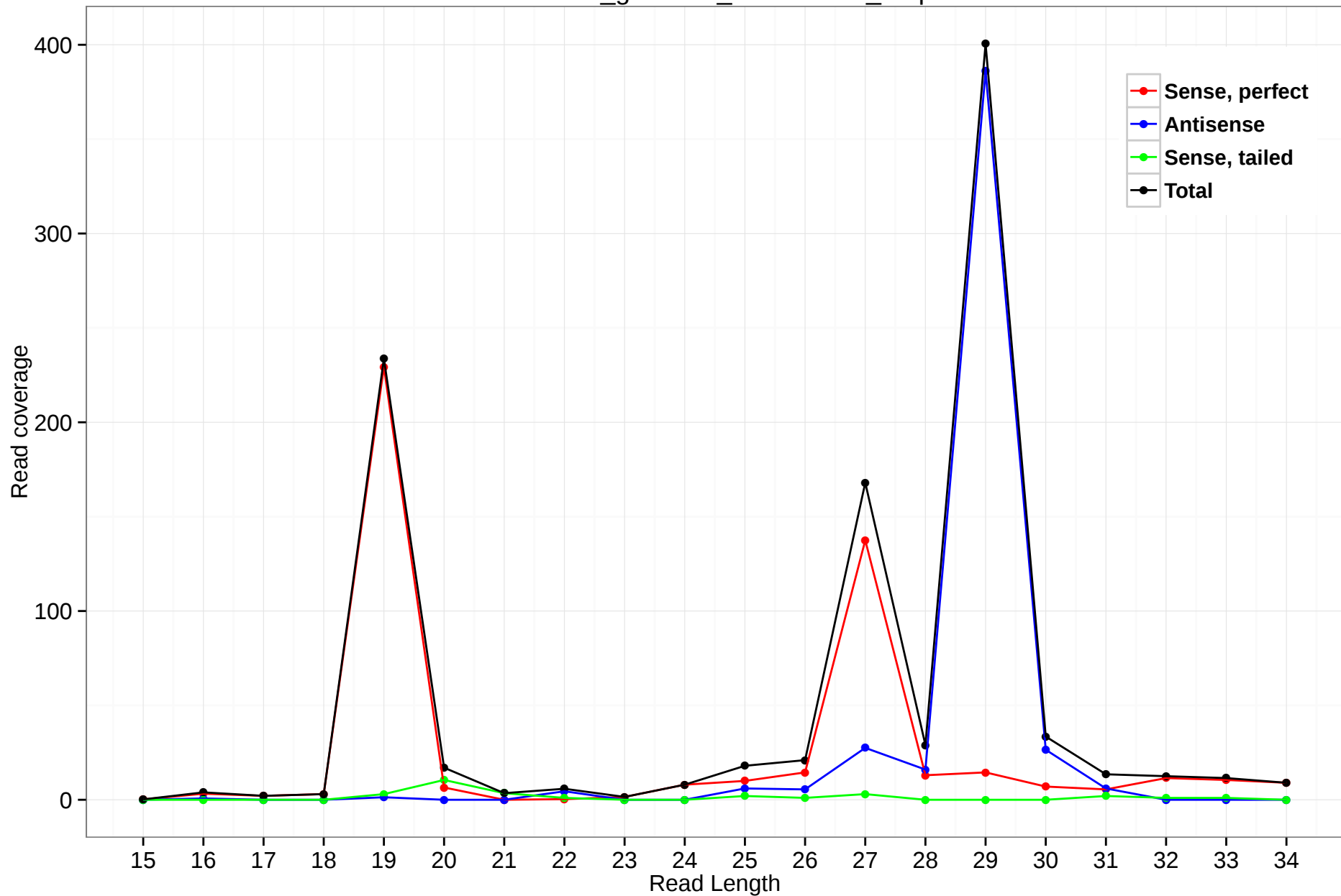
rheMac3_genscan_chr15.1822_8.5p
