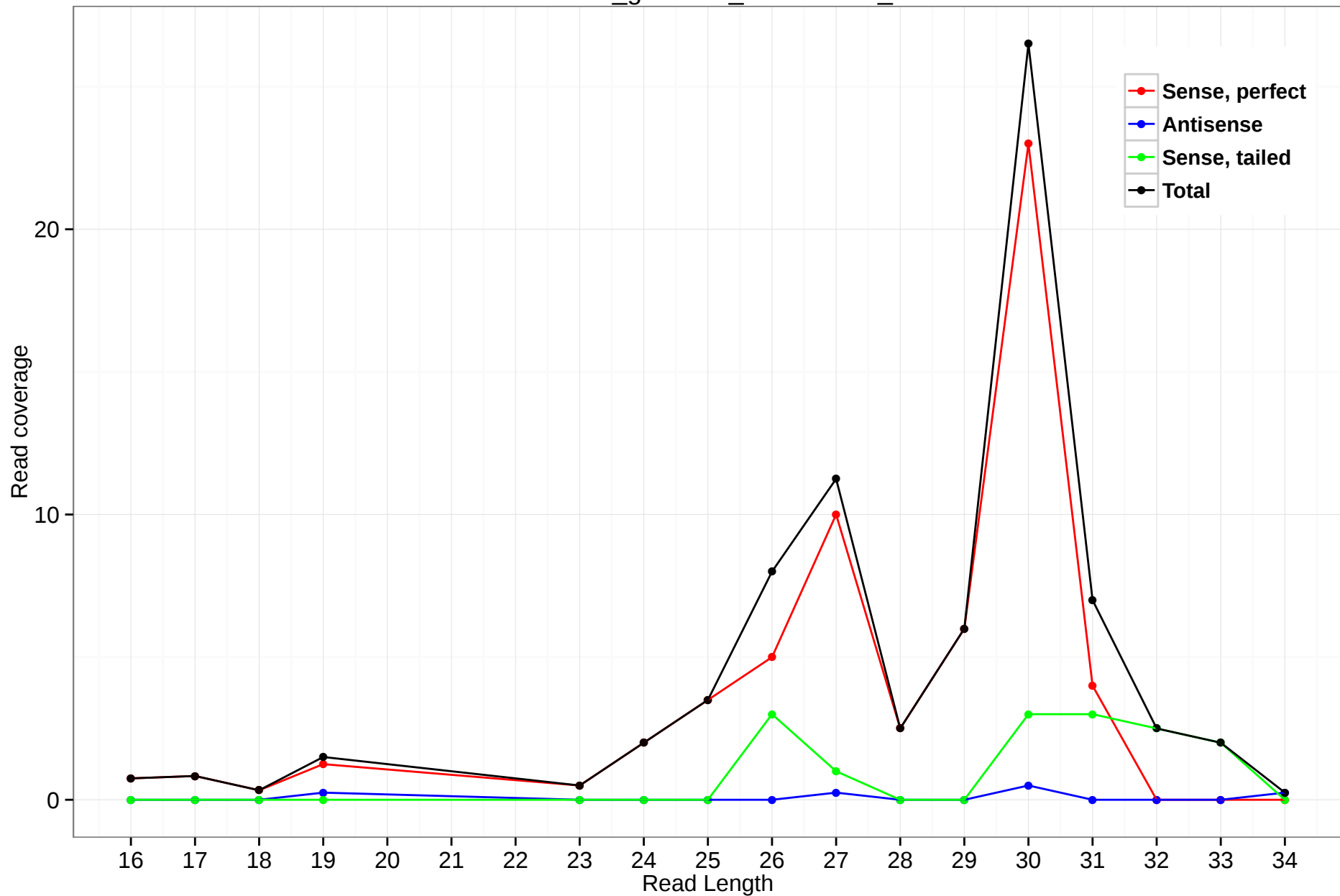
rheMac3_genscan_chr15.1822_7
