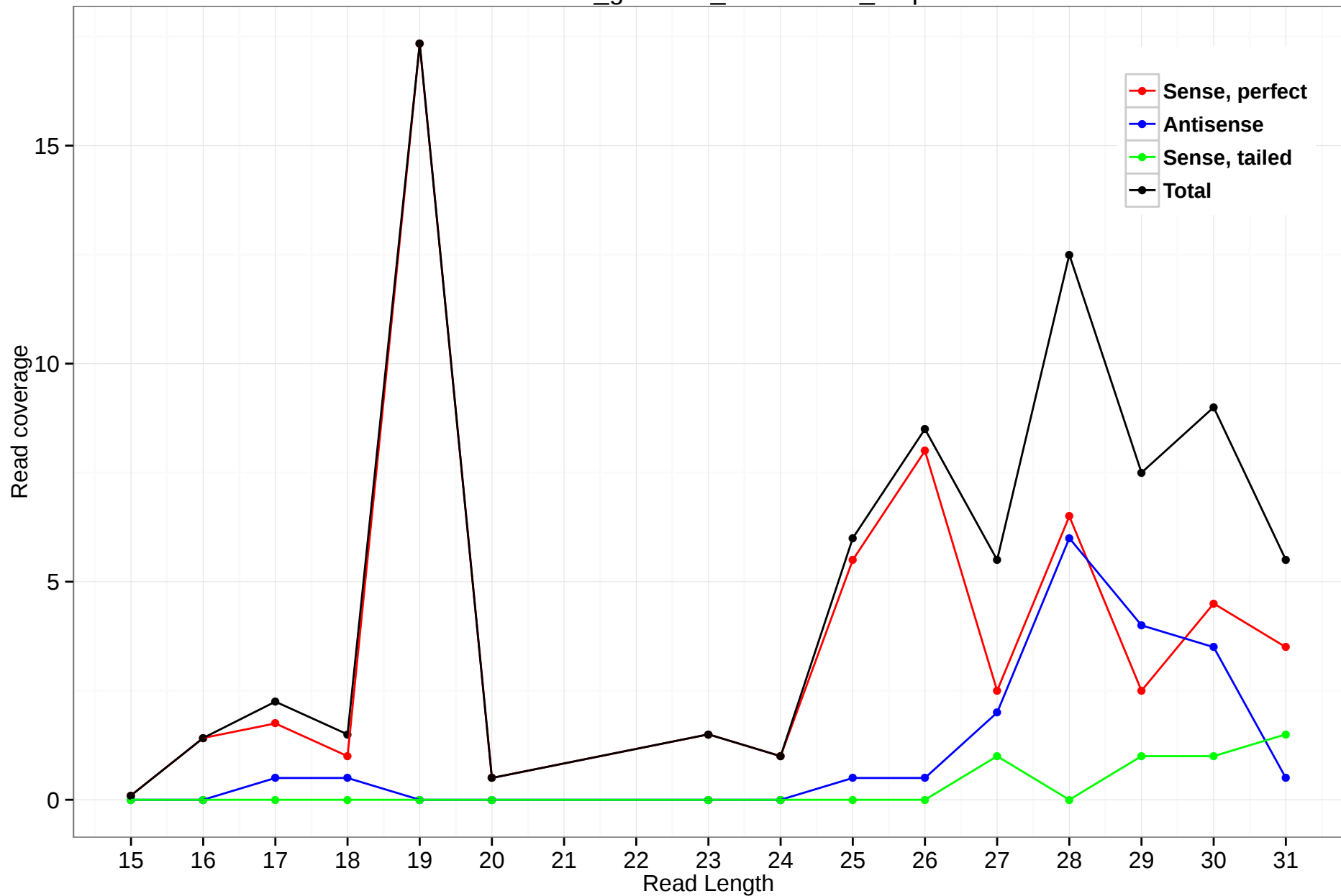
rheMac3_genscan_chr15.1822_6.5p
