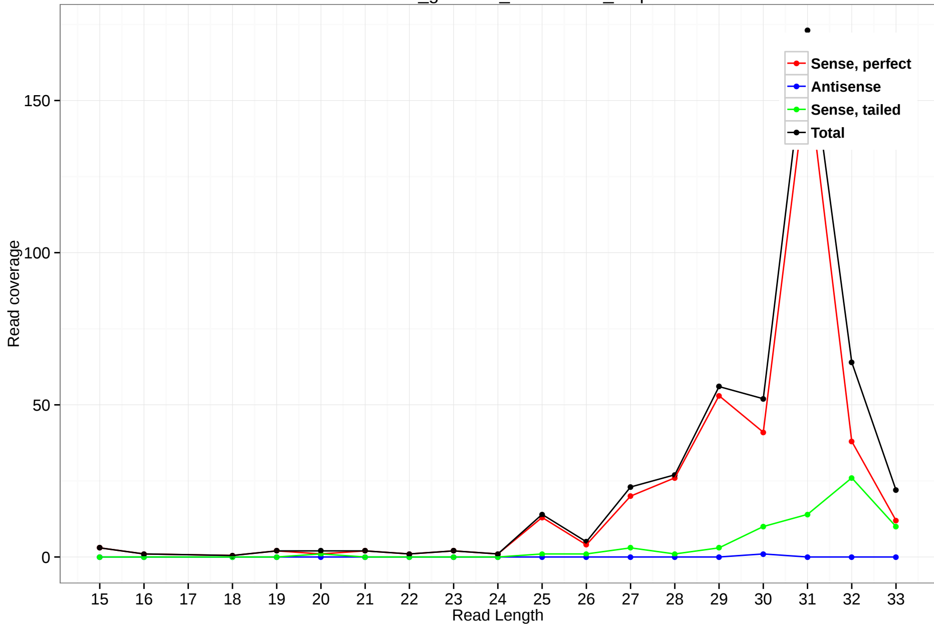
rheMac3_genscan_chr15.1822_4.3p
