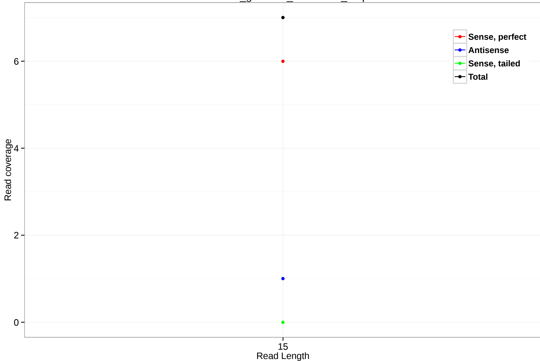
rheMac3_genscan_chr15.179_0.3p
