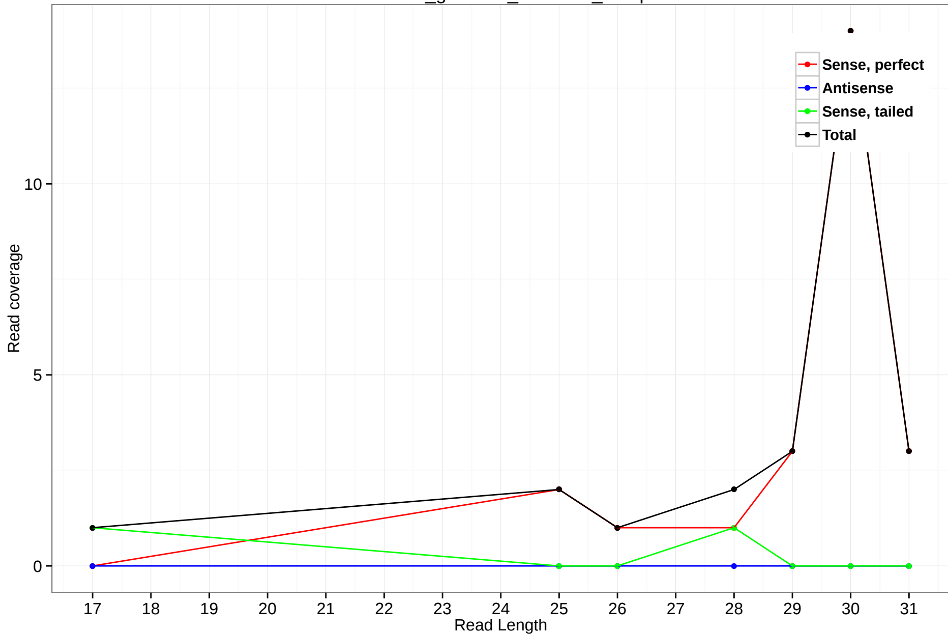
rheMac3_genscan_chr15.16_19.3p
