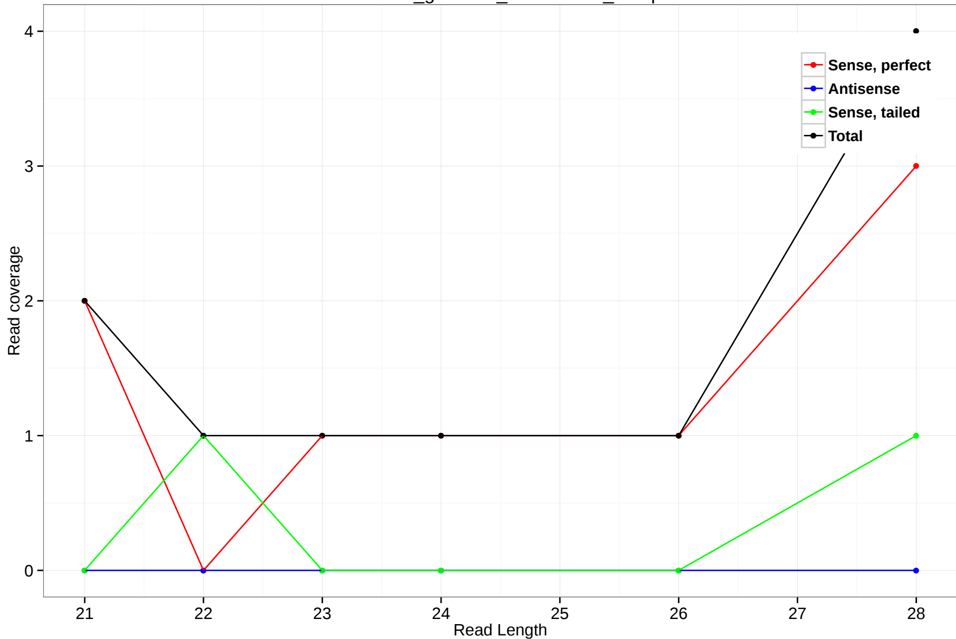
rheMac3_genscan_chr15.1621_16.3p
