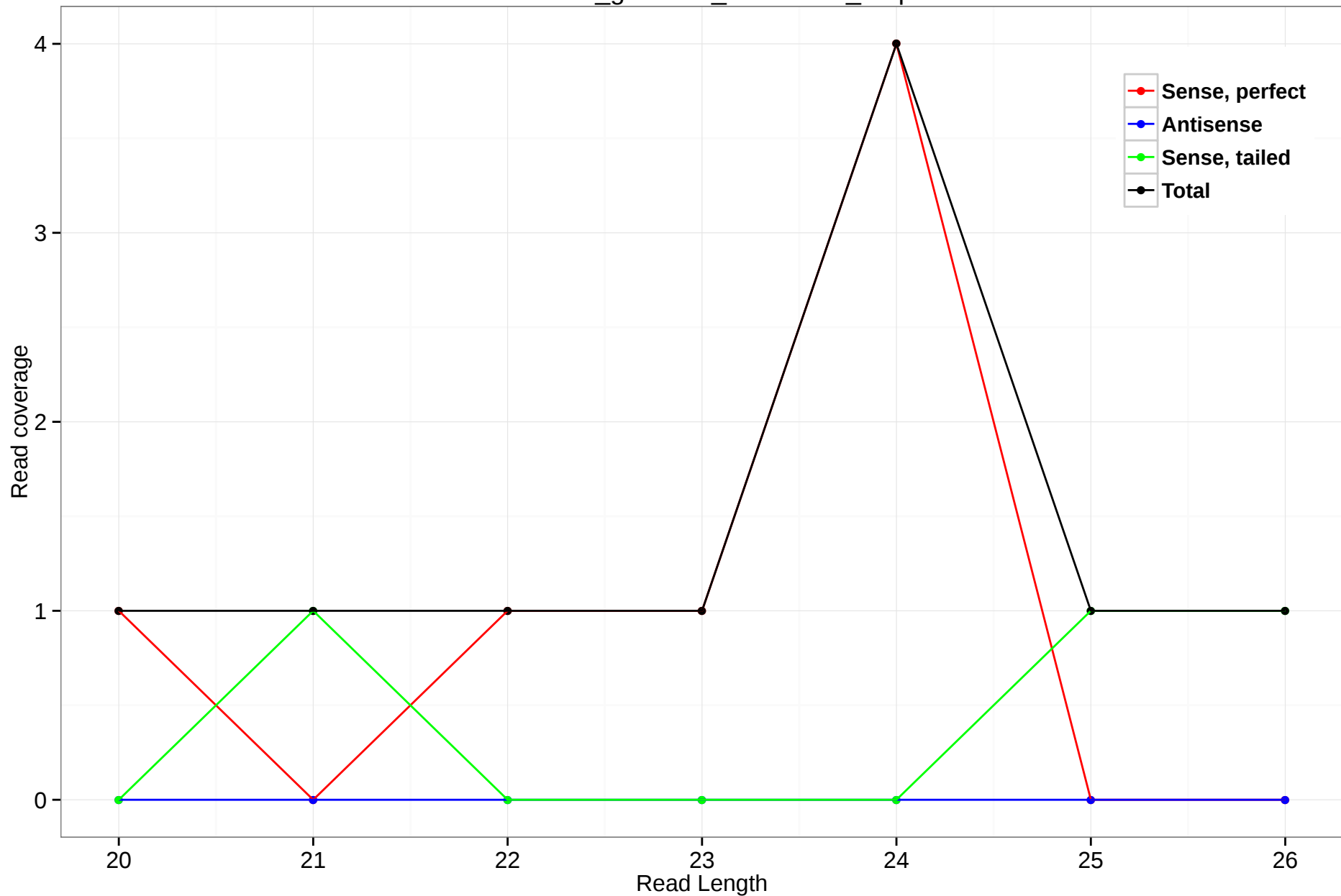
rheMac3_genscan_chr15.145_4.3p
