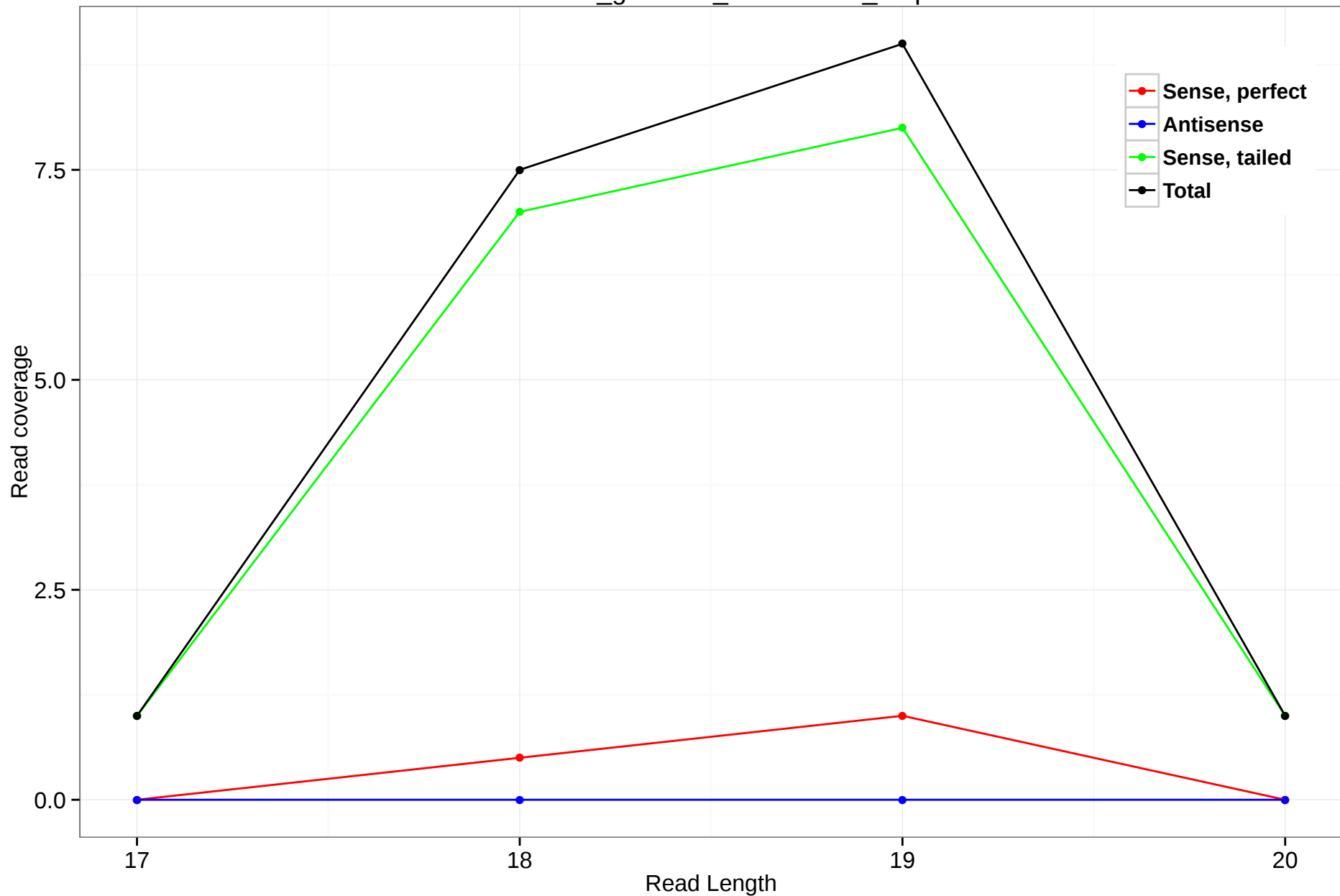
rheMac3_genscan_chr15.1382_1.3p
