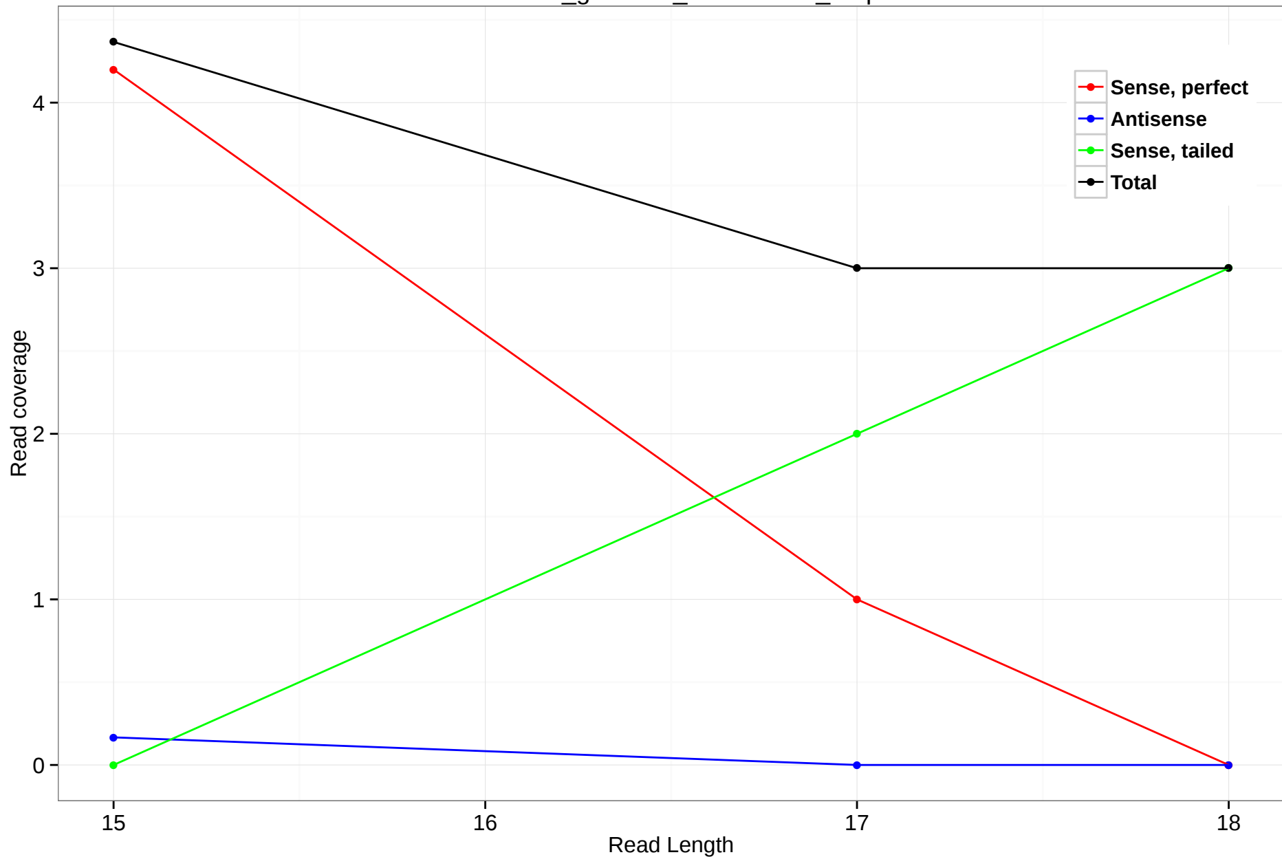
rheMac3_genscan_chr15.1323_4.5p
