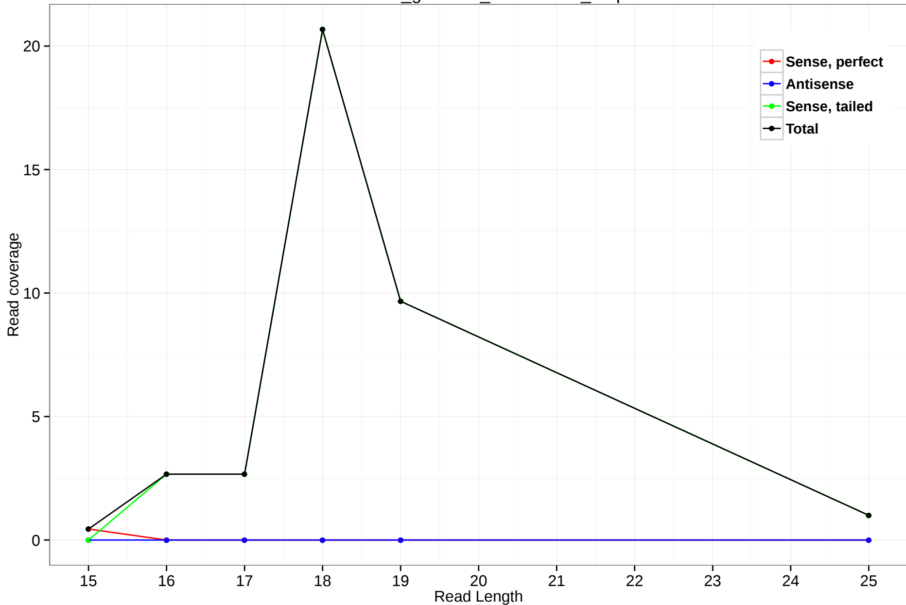
rheMac3_genscan_chr15.1241_6.3p
