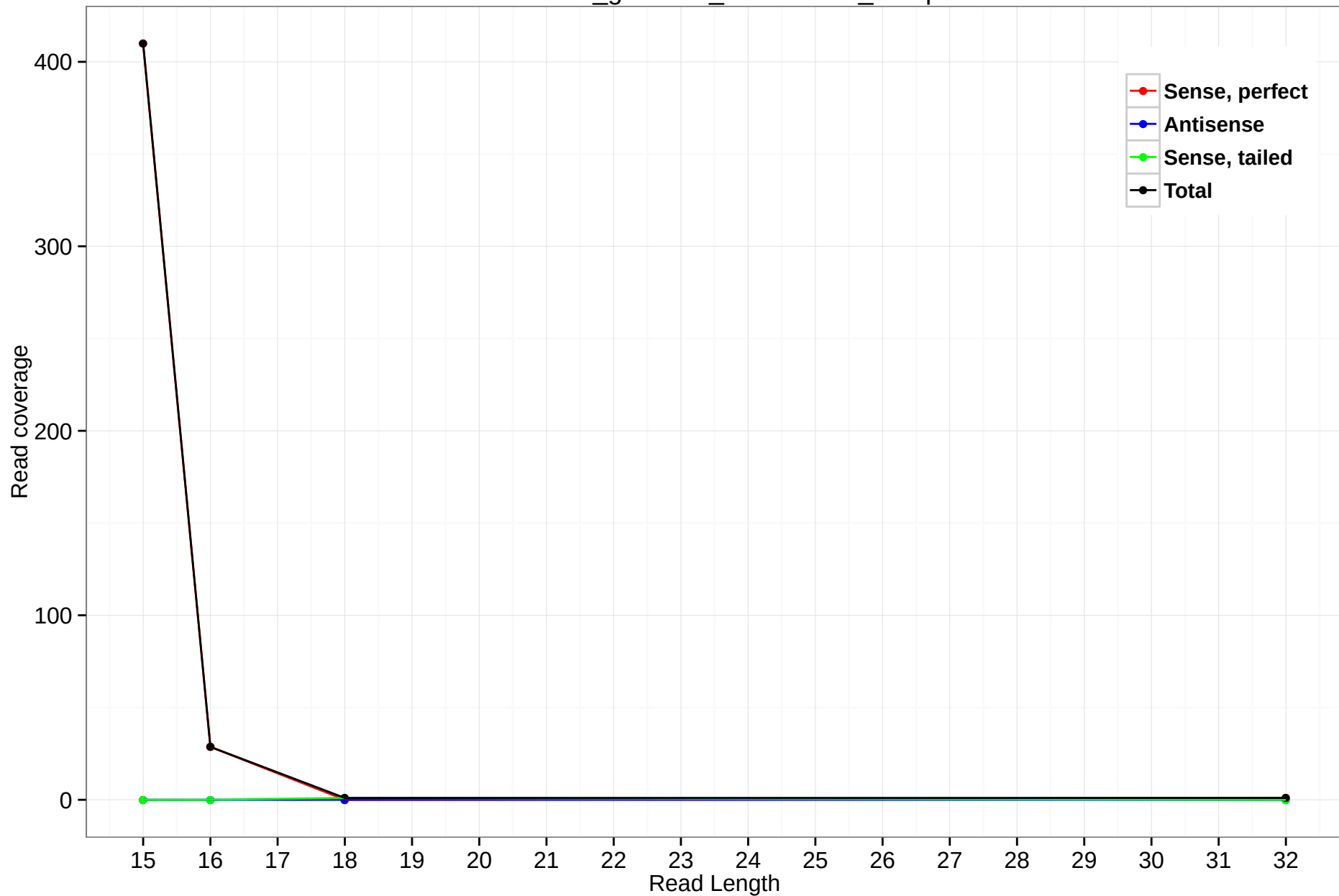
rheMac3_genscan_chr15.1217_16.3p
