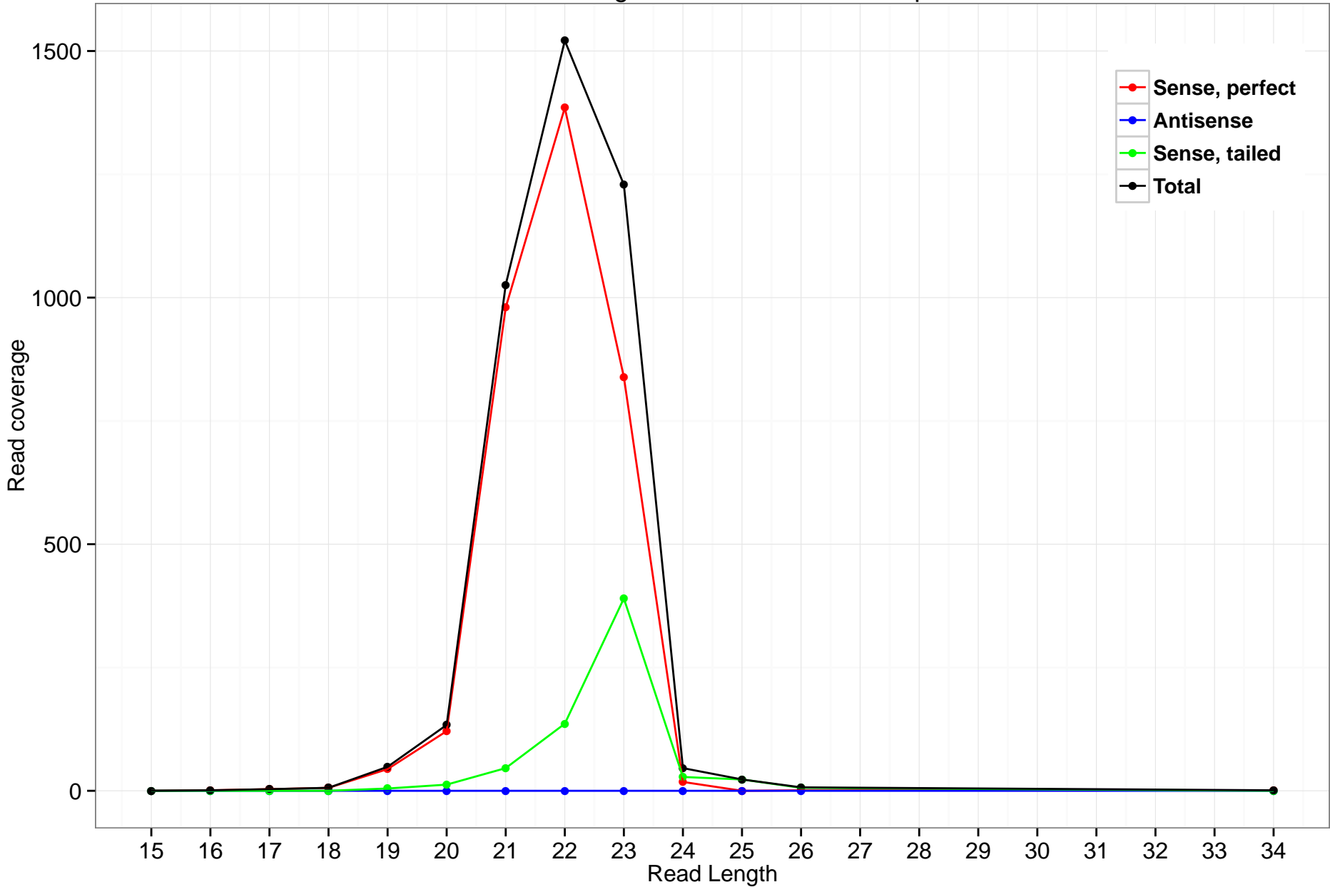
rheMac3_genscan_chr15.1186_1.5p
