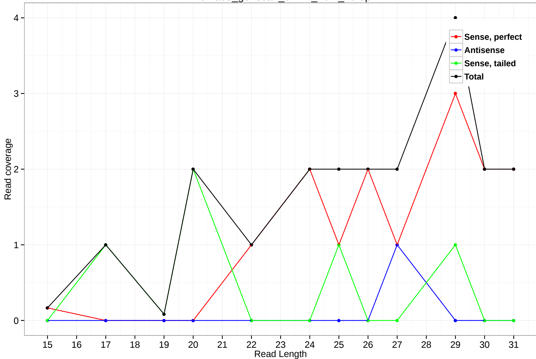
rheMac3_genscan_chr14_76.4_10.5p
