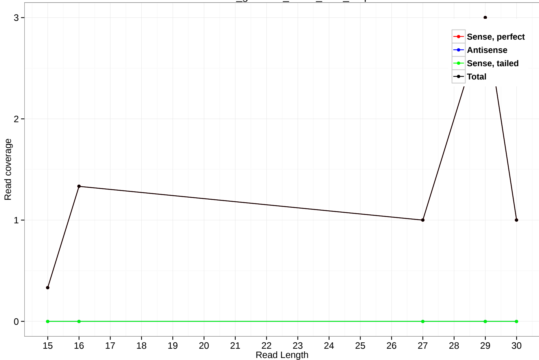
rheMac3_genscan_chr14_75.5_4.3p
