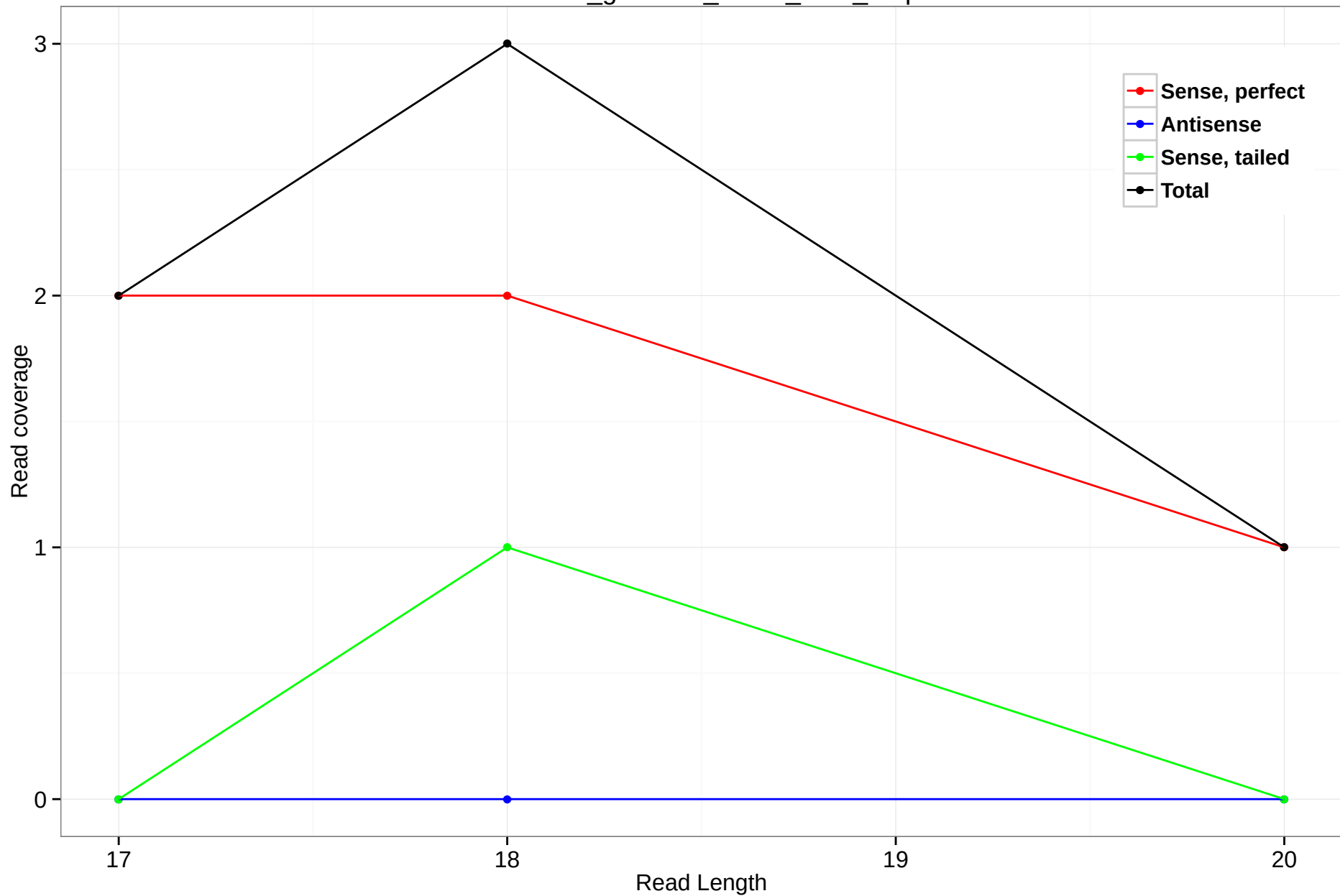
rheMac3_genscan_chr14_75.1_0.5p
