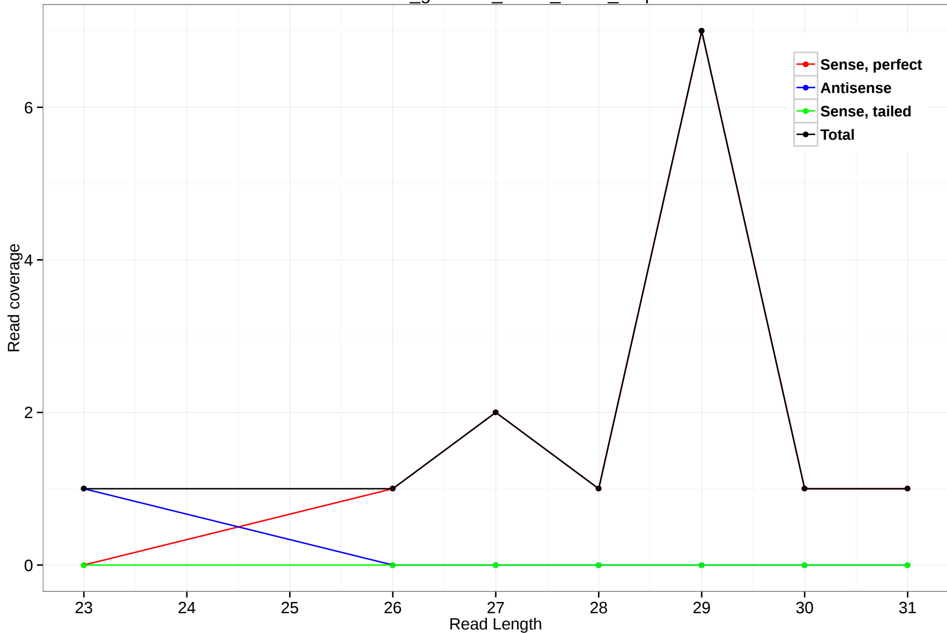
rheMac3_genscan_chr14_75.11_2.5p
