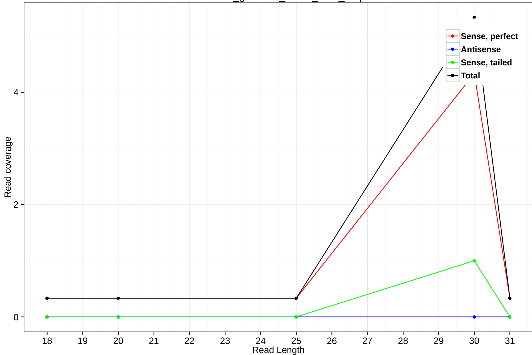
rheMac3_genscan_chr14_74.2_1.3p
