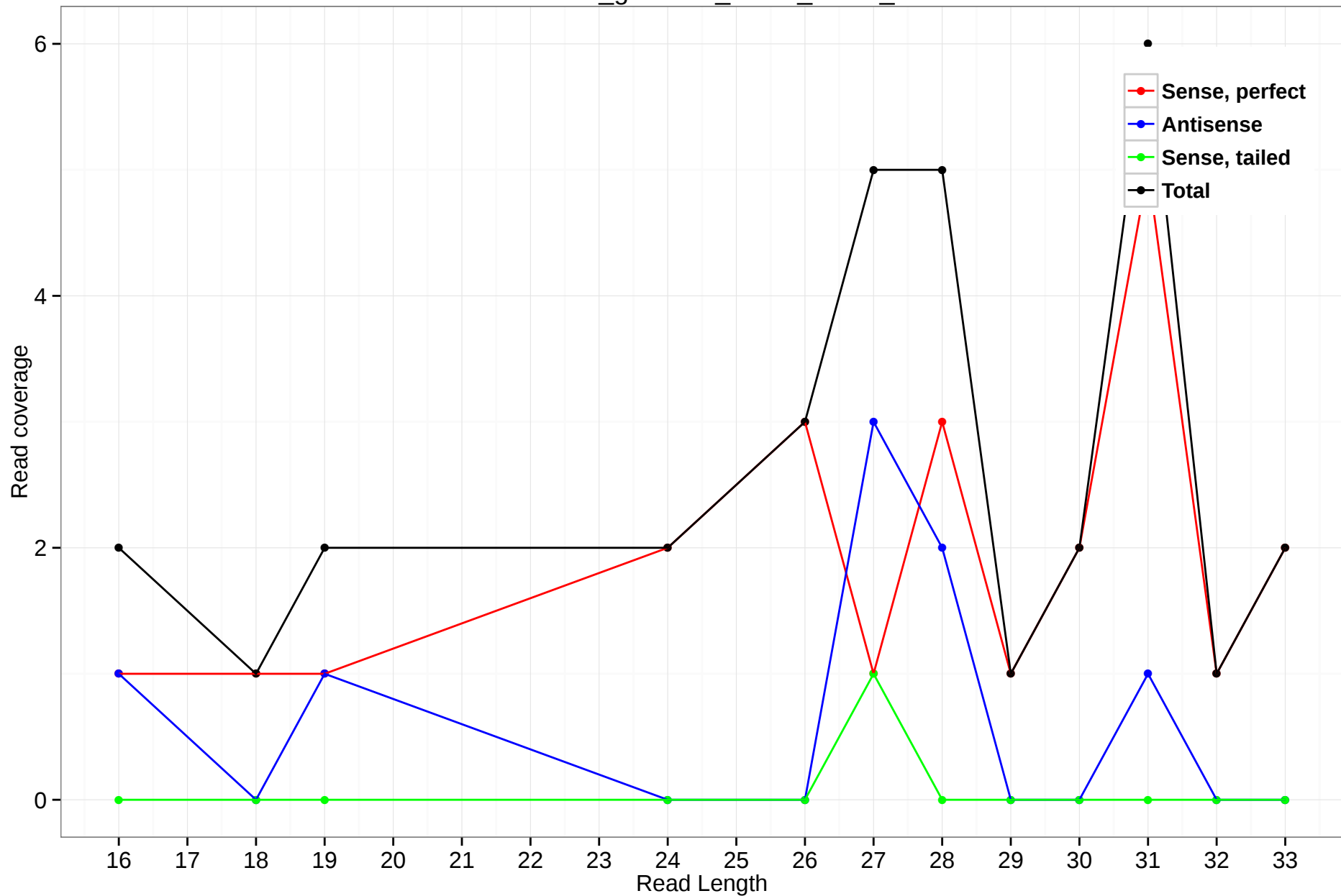
rheMac3_genscan_chr14_73.11_9
