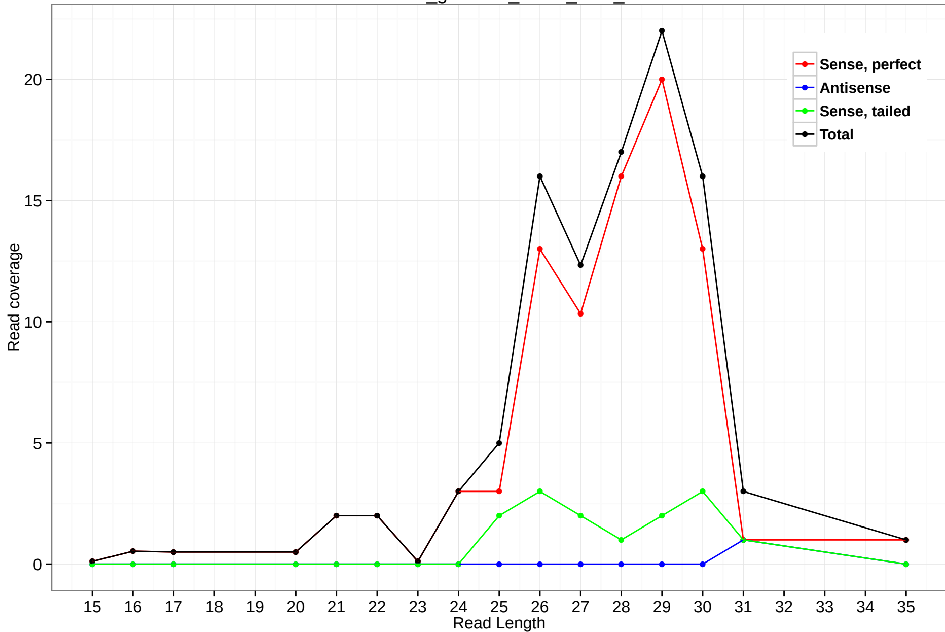
rheMac3_genscan_chr14_72.6_10
