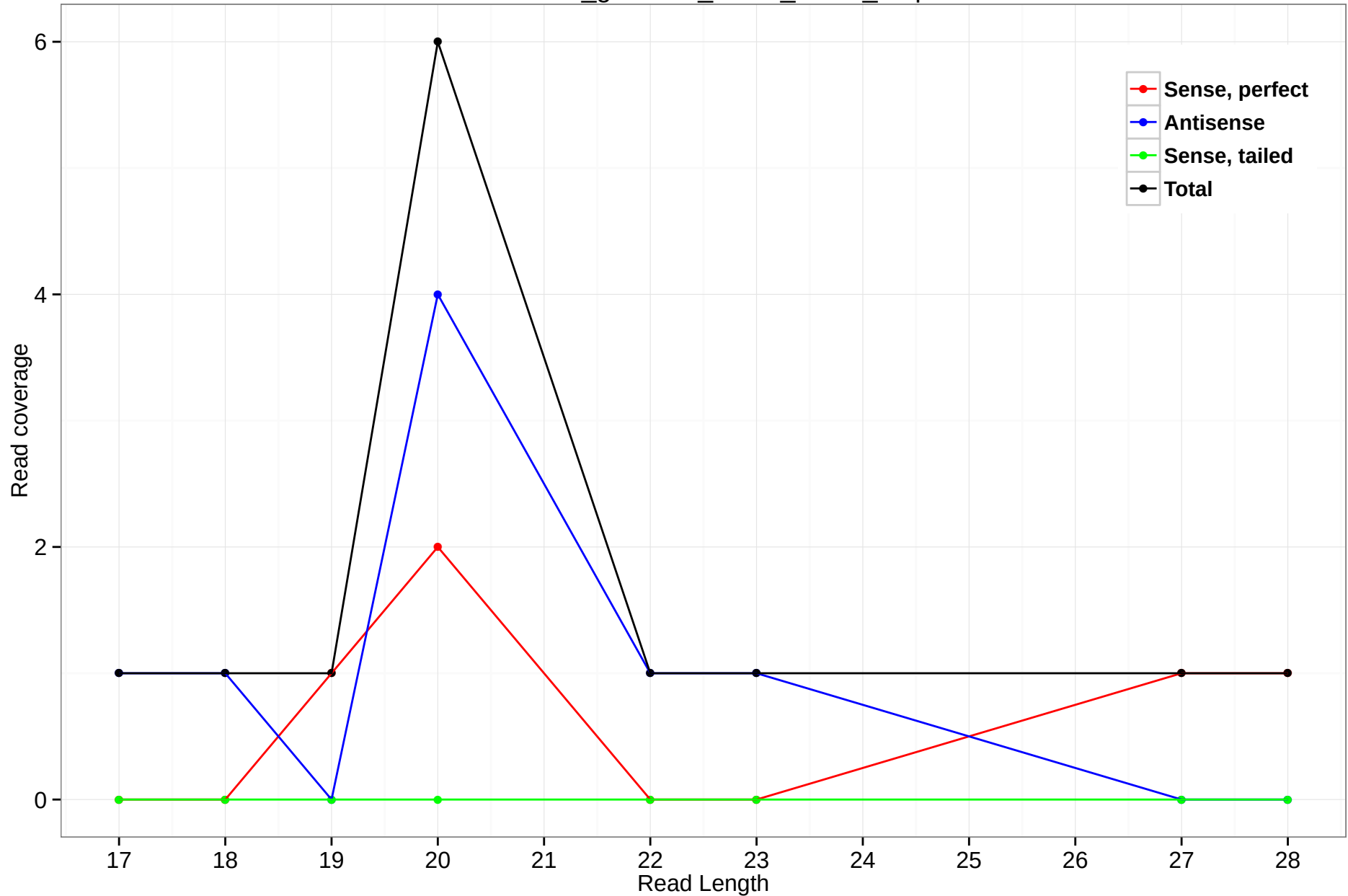
rheMac3_genscan_chr14_70.51_0.5p
