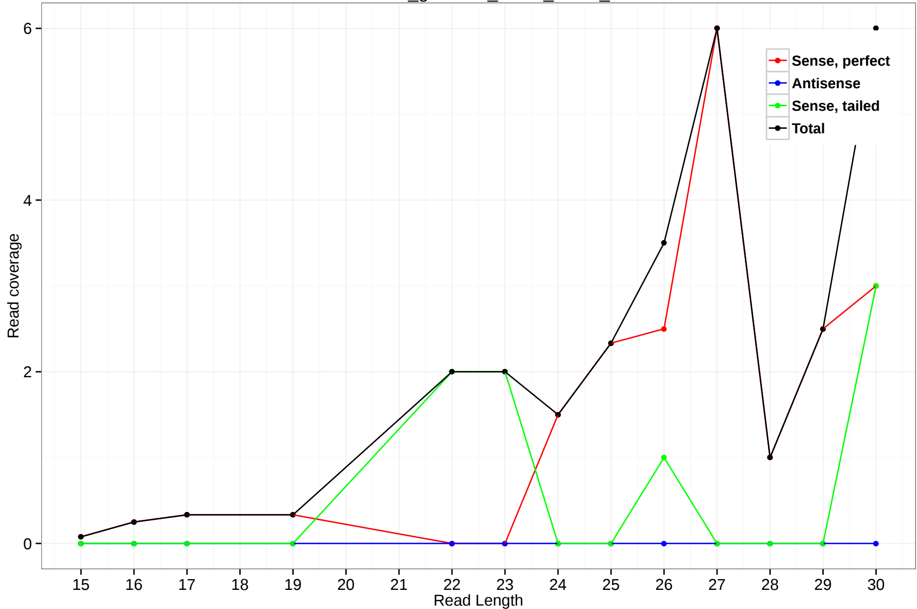
rheMac3_genscan_chr14_70.37_2
