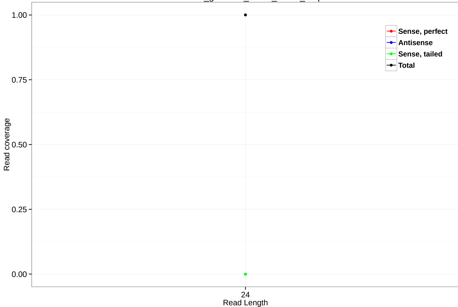
rheMac3_genscan_chr14_70.34_1.5p
