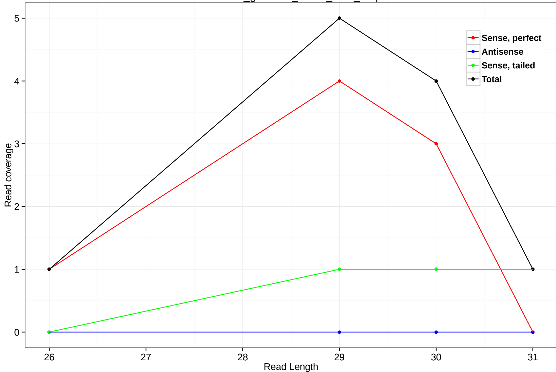
rheMac3_genscan_chr14_55.8_9.3p
