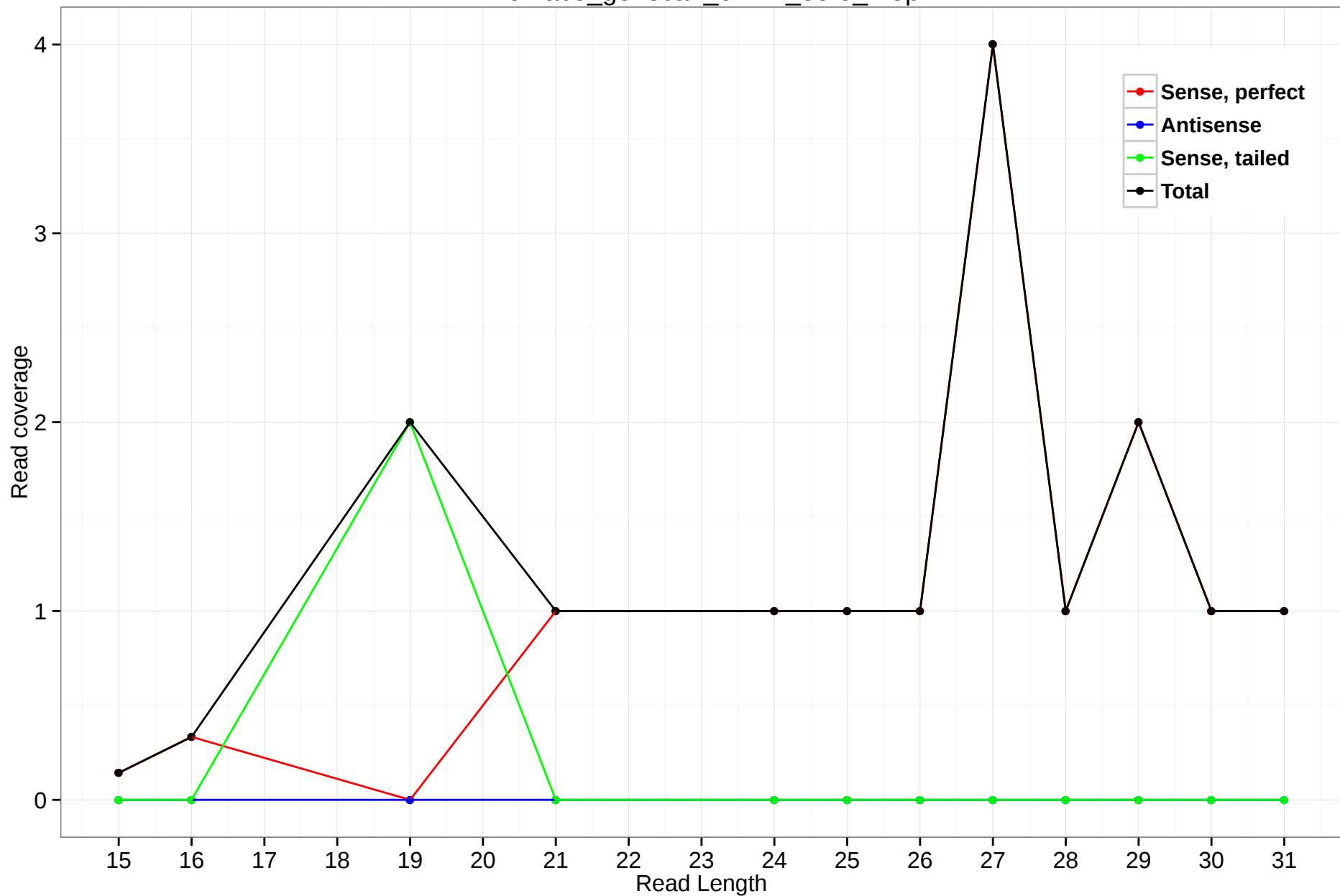
rheMac3_genscan_chr14_55.8_2.5p
