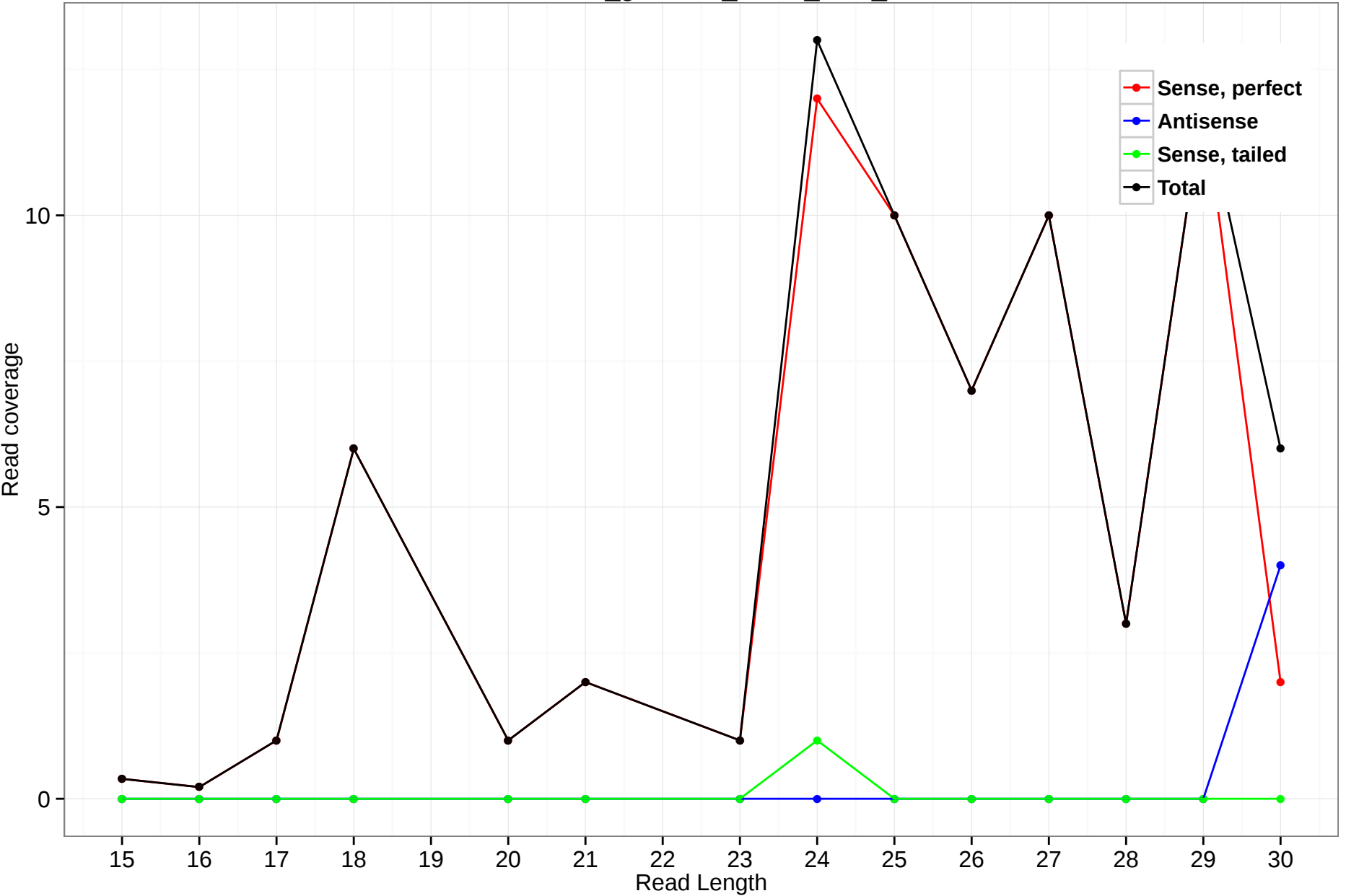
rheMac3_genscan_chr14_55.8_0
