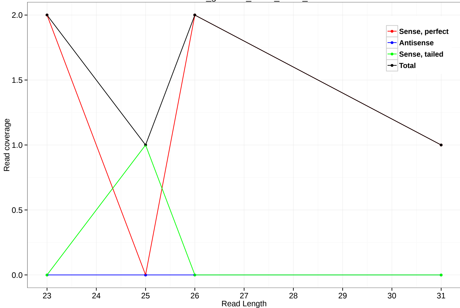
rheMac3_genscan_chr14_55.10_11
