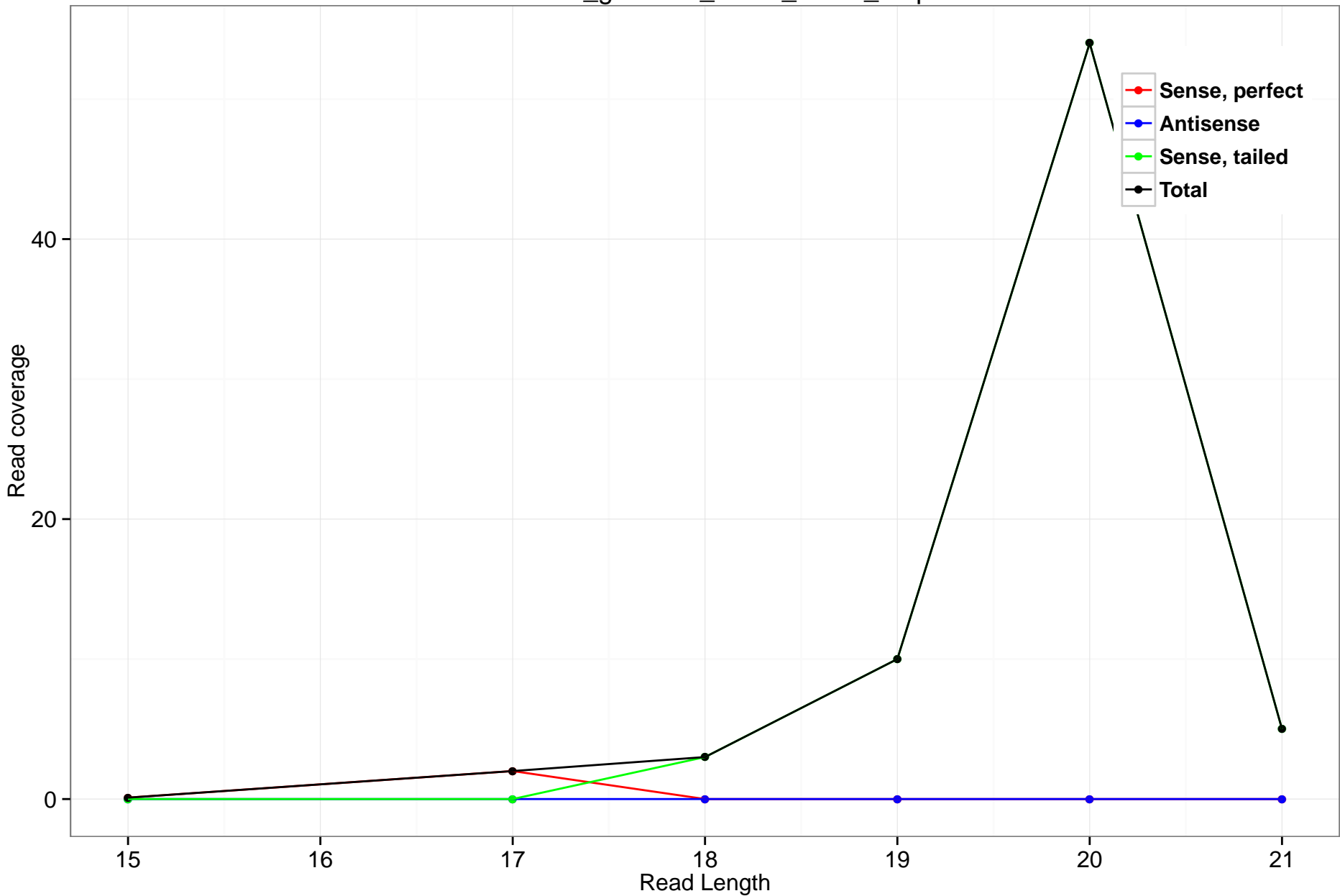
rheMac3_genscan_chr14_51.18_9.5p
