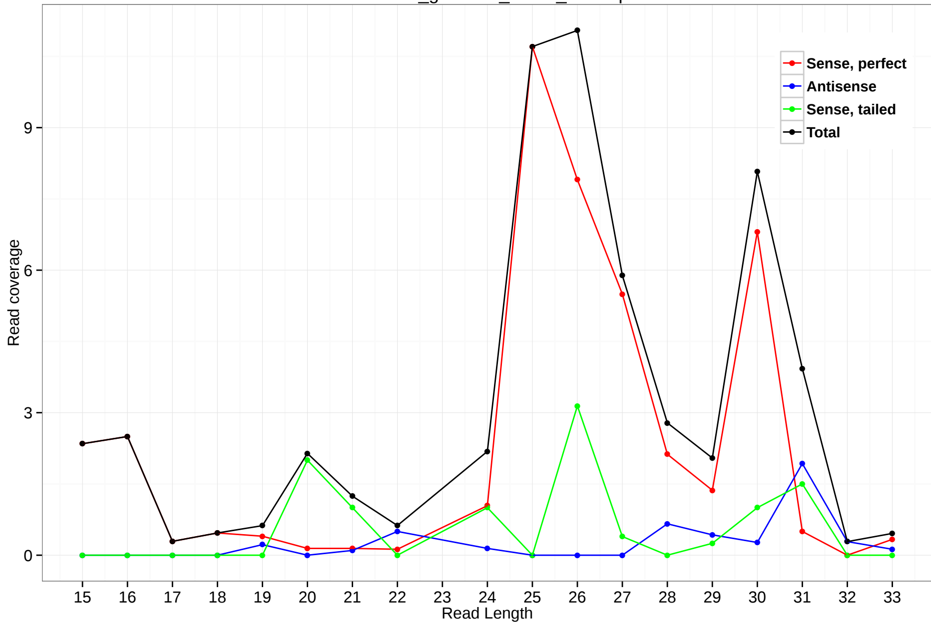
rheMac3_genscan_chr14_44.5.5p
