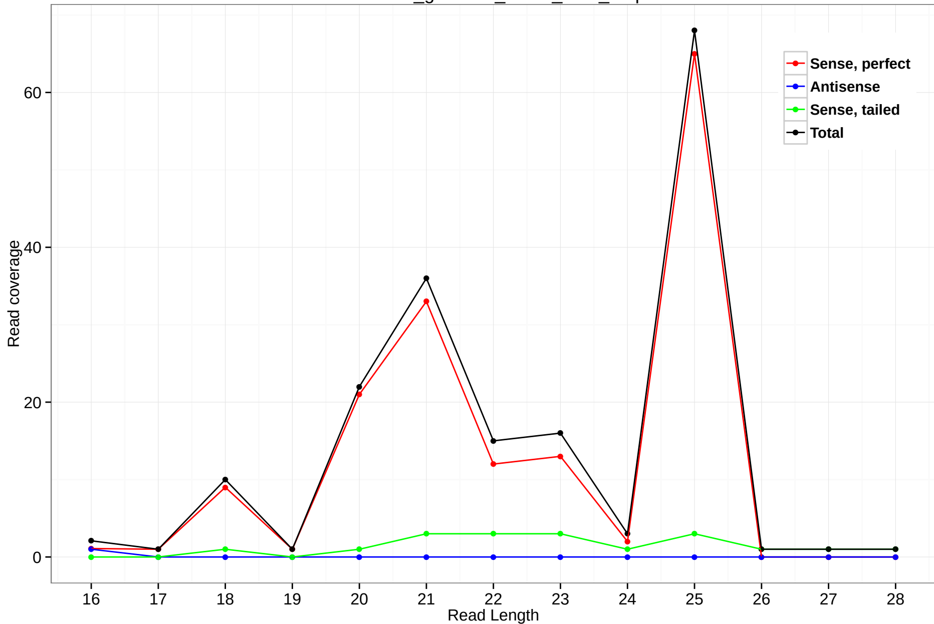
rheMac3_genscan_chr14_44.1_0.3p
