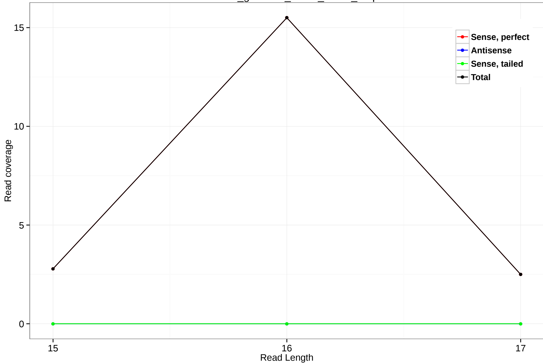
rheMac3_genscan_chr14_43.45_8.3p
