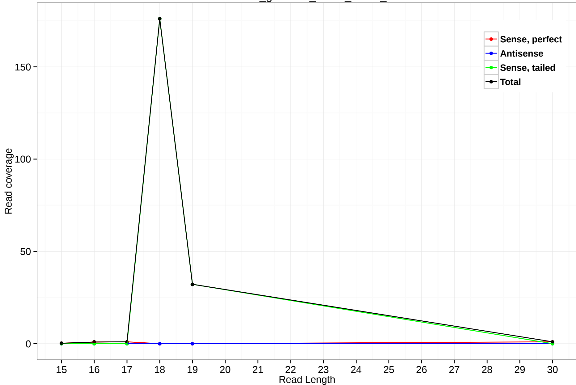
rheMac3_genscan_chr14_43.45_19
