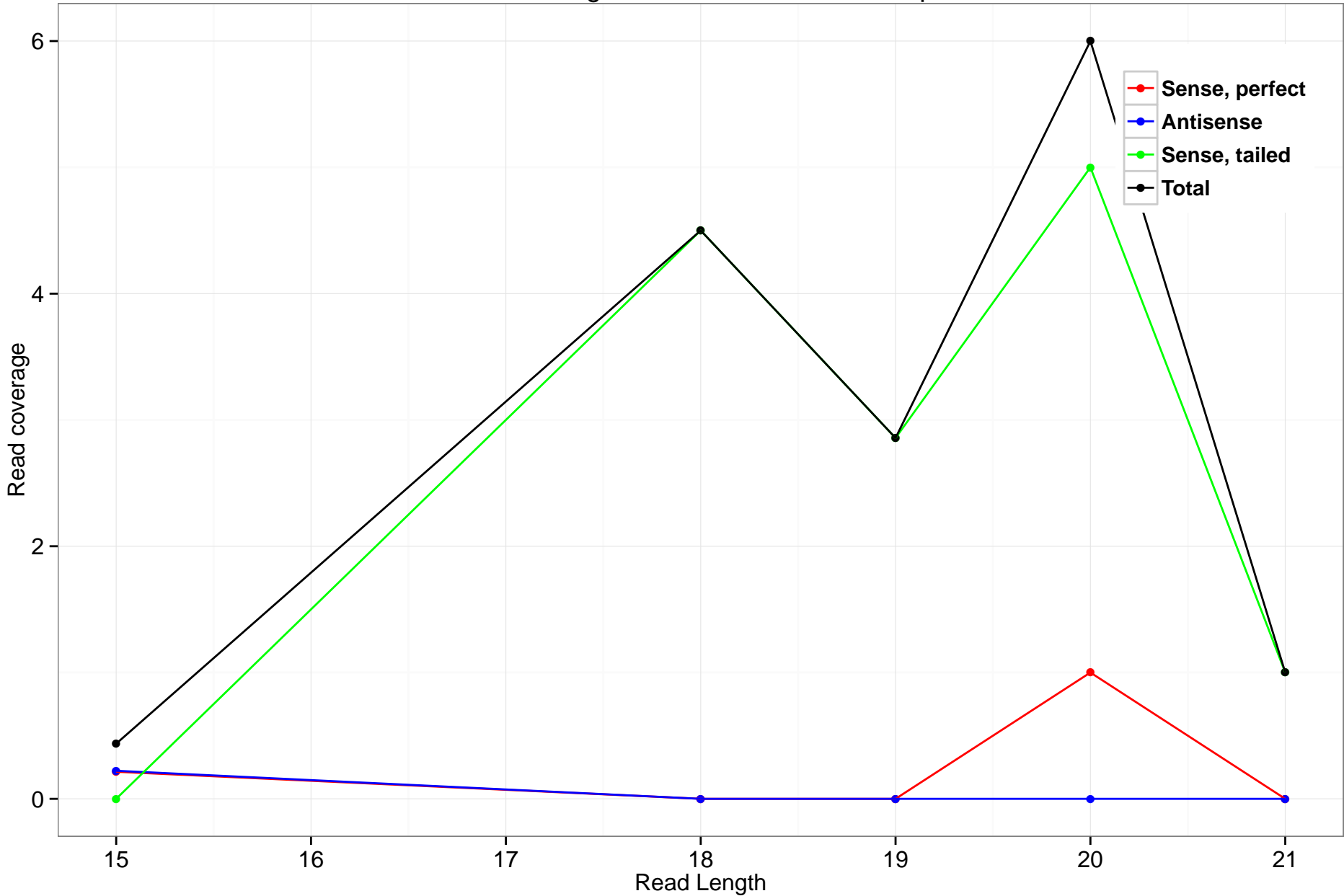
rheMac3_genscan_chr14_43.44_19.3p
