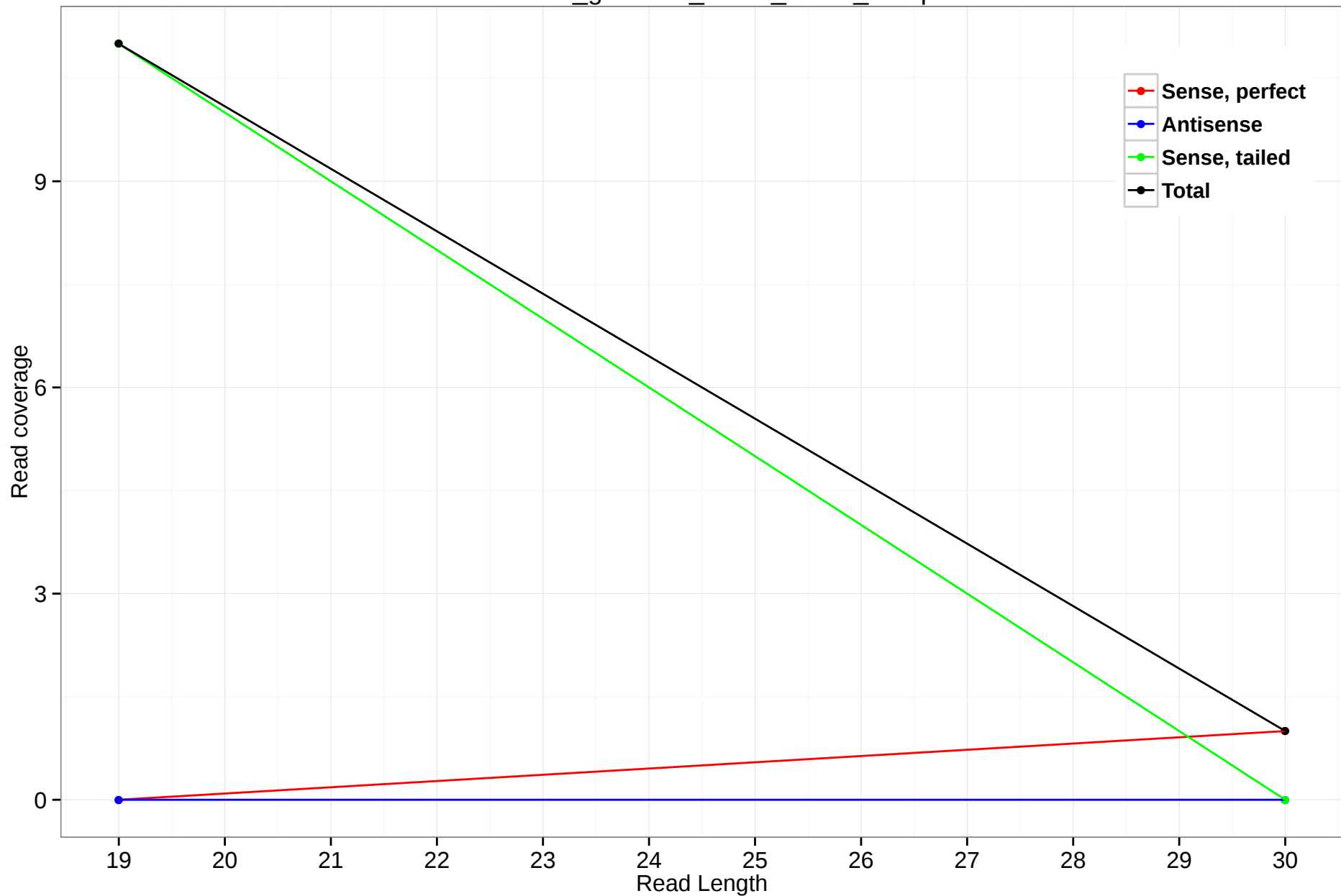
rheMac3_genscan_chr14_42.82_26.3p
