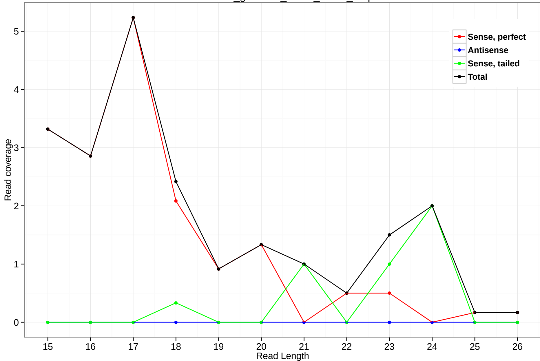
rheMac3_genscan_chr14_42.28_2.3p
