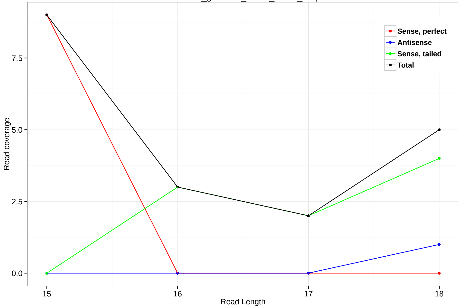
rheMac3_genscan_chr14_42.25_2.5p
