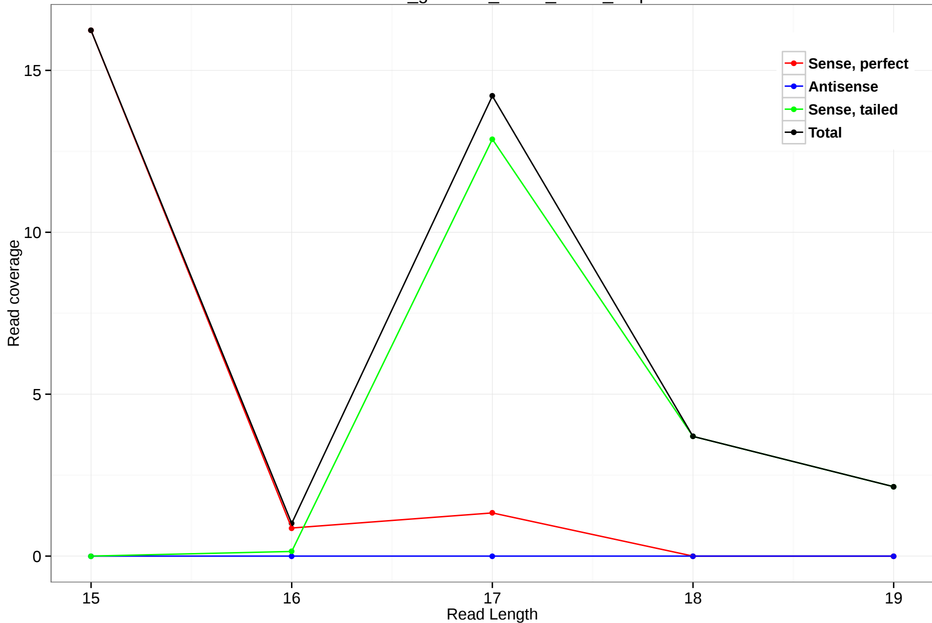
rheMac3_genscan_chr14_29.67_0.5p
