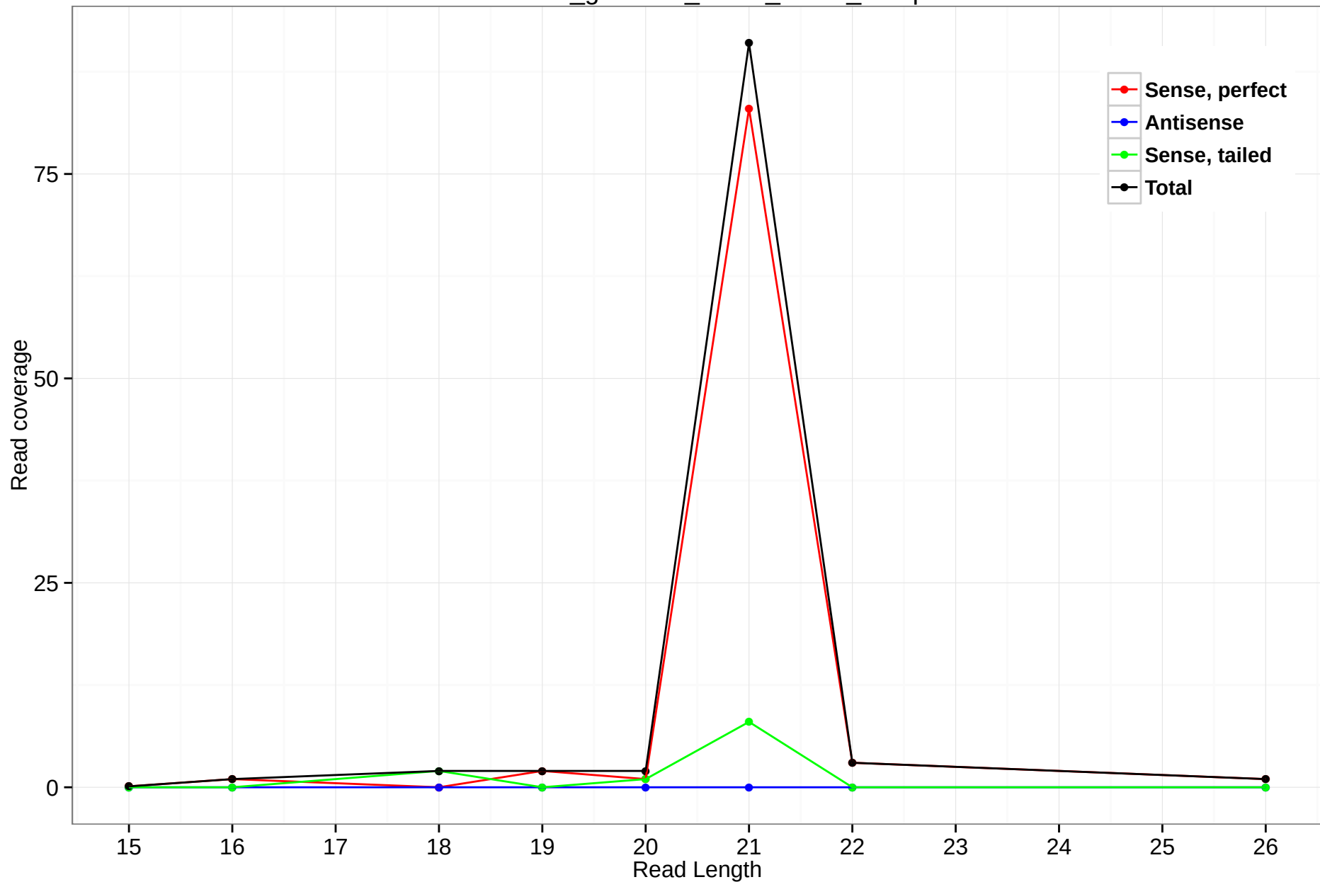
rheMac3_genscan_chr14_29.48_10.5p
