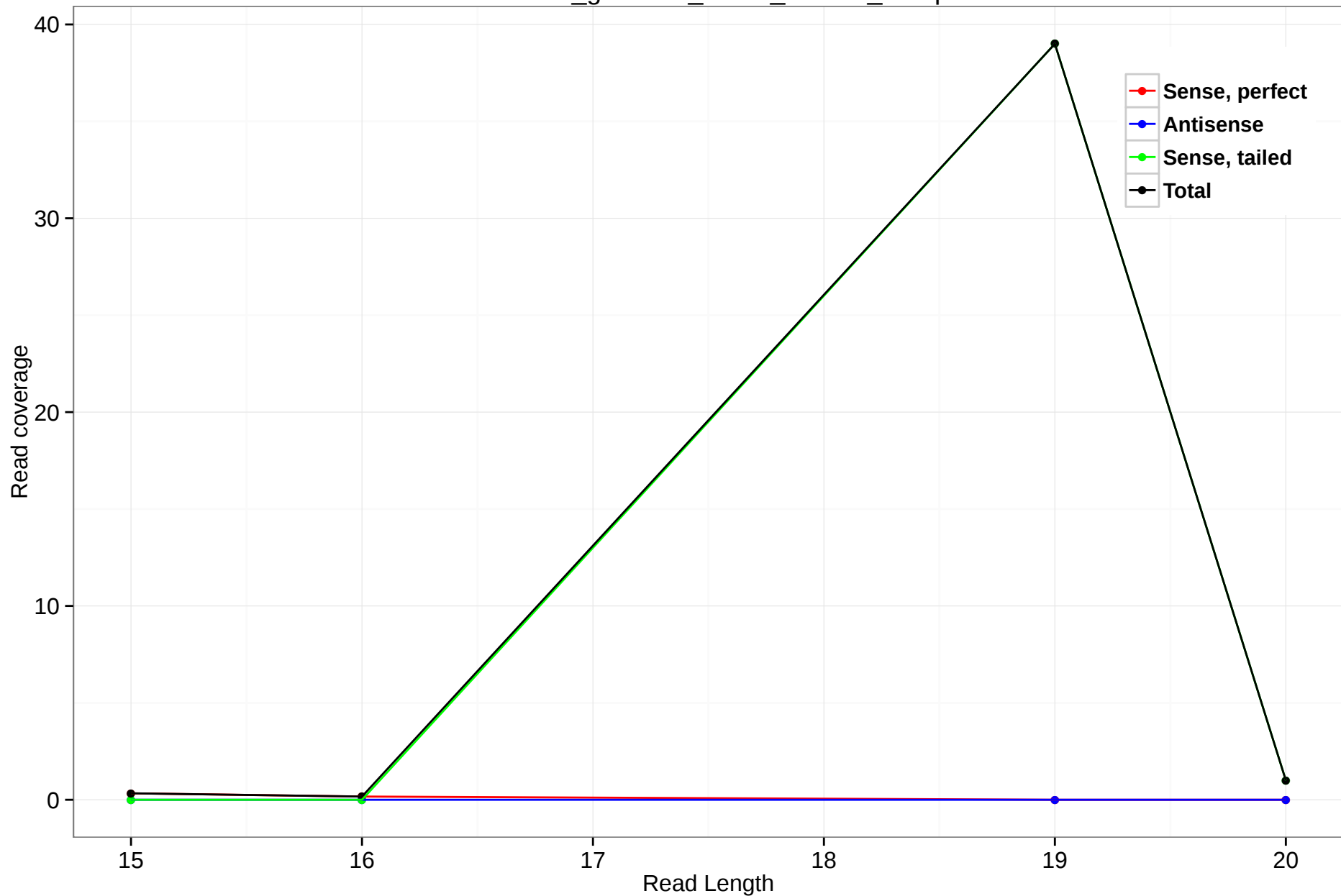
rheMac3_genscan_chr14_29.109_11.5p
