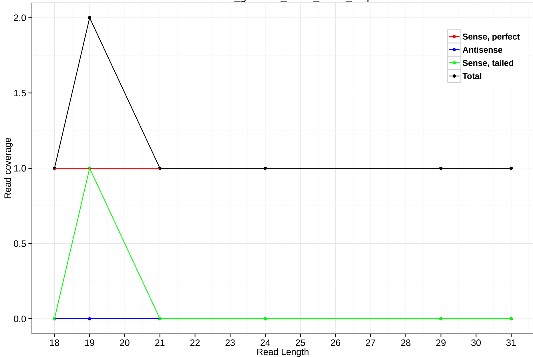
rheMac3_genscan_chr14_24.61_9.5p
