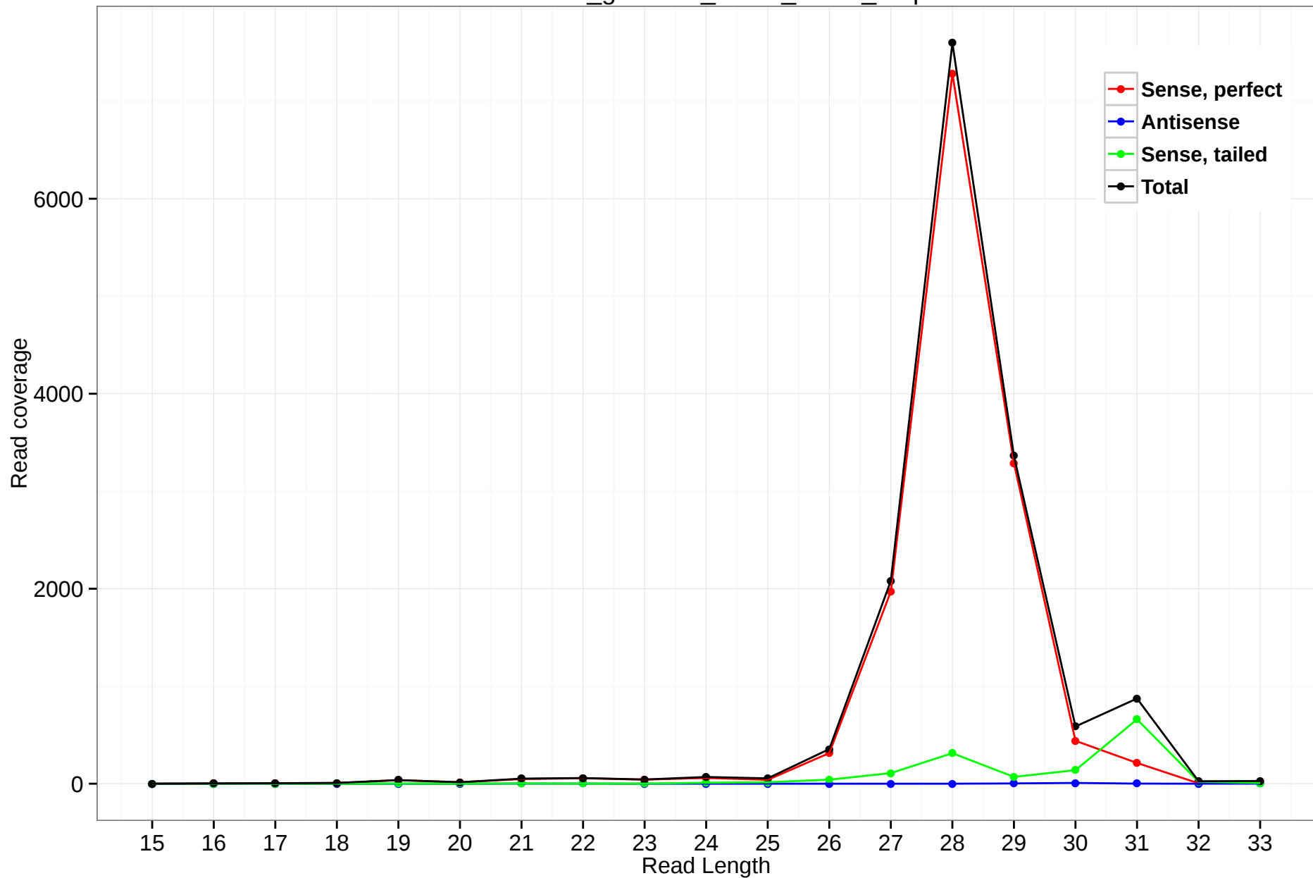
rheMac3_genscan_chr14_24.61_3.5p
