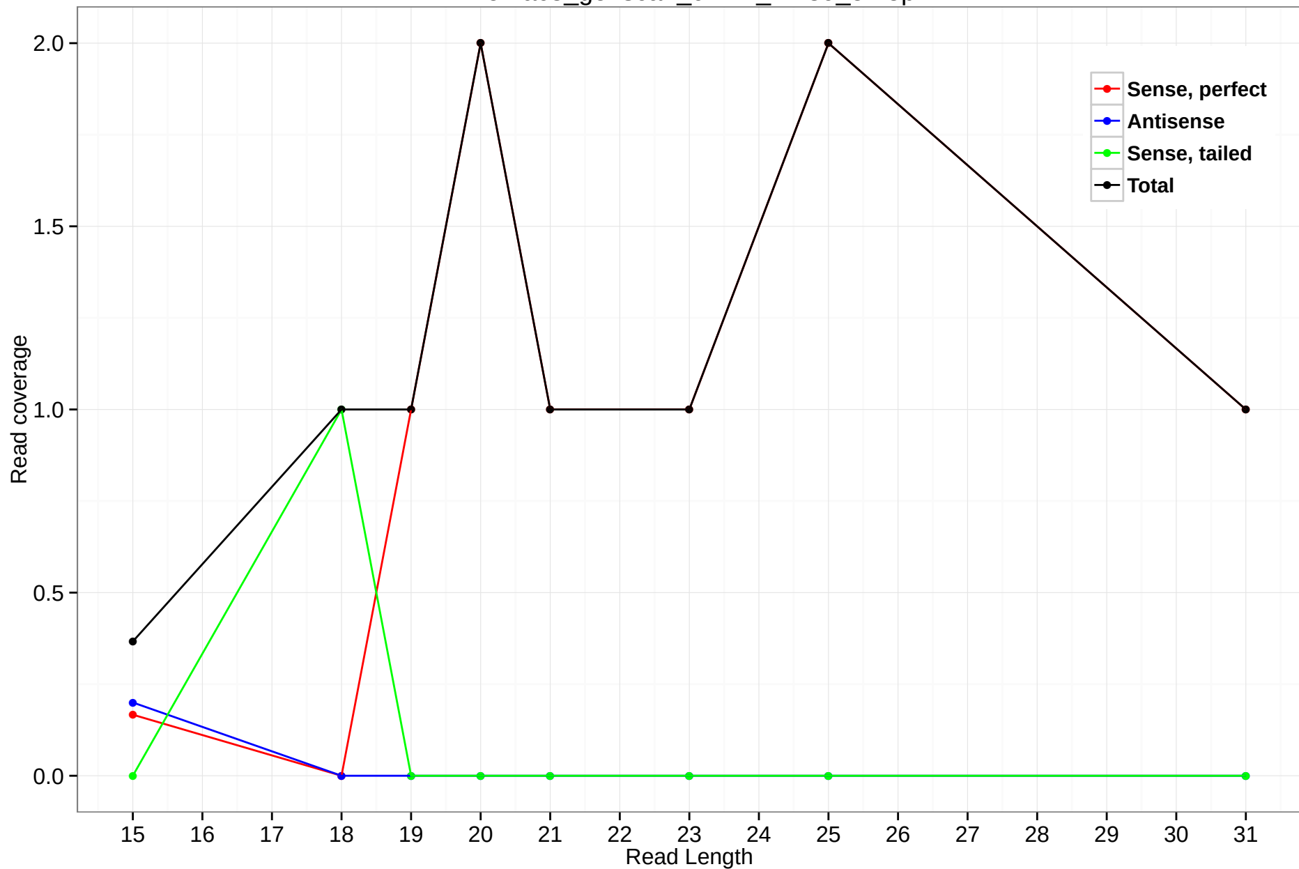
rheMac3_genscan_chr14_24.39_51.5p
