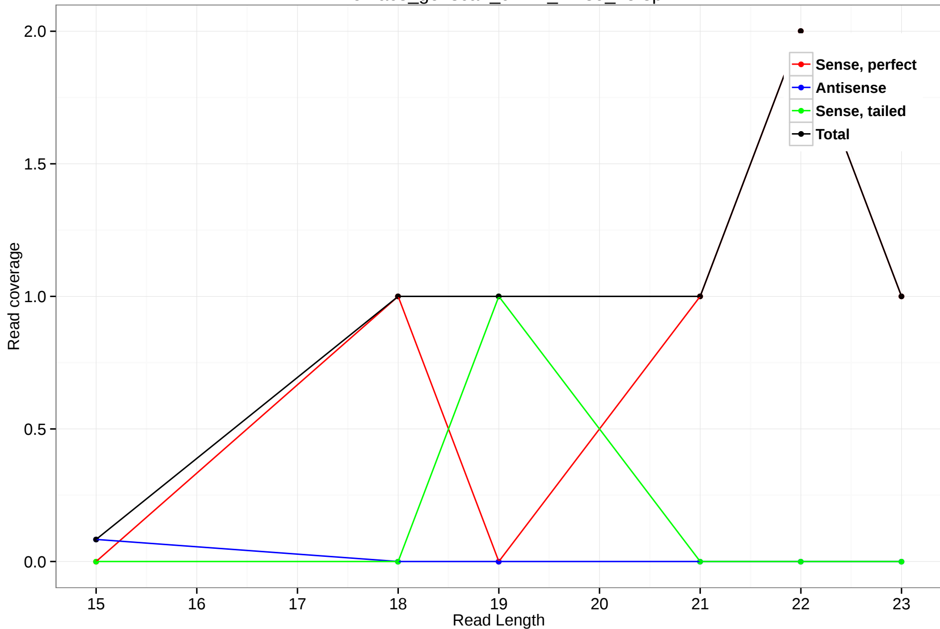
rheMac3_genscan_chr14_24.39_45.3p
