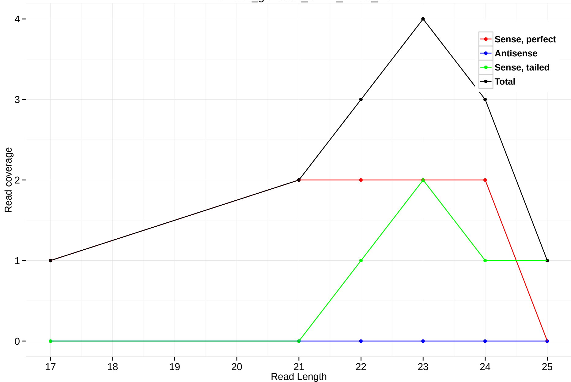
rheMac3_genscan_chr14_24.39_43
