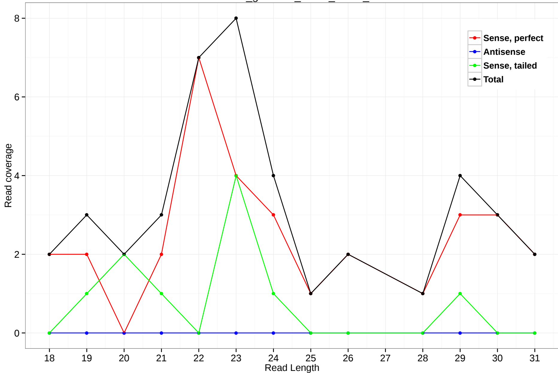
rheMac3_genscan_chr14_24.39_37
