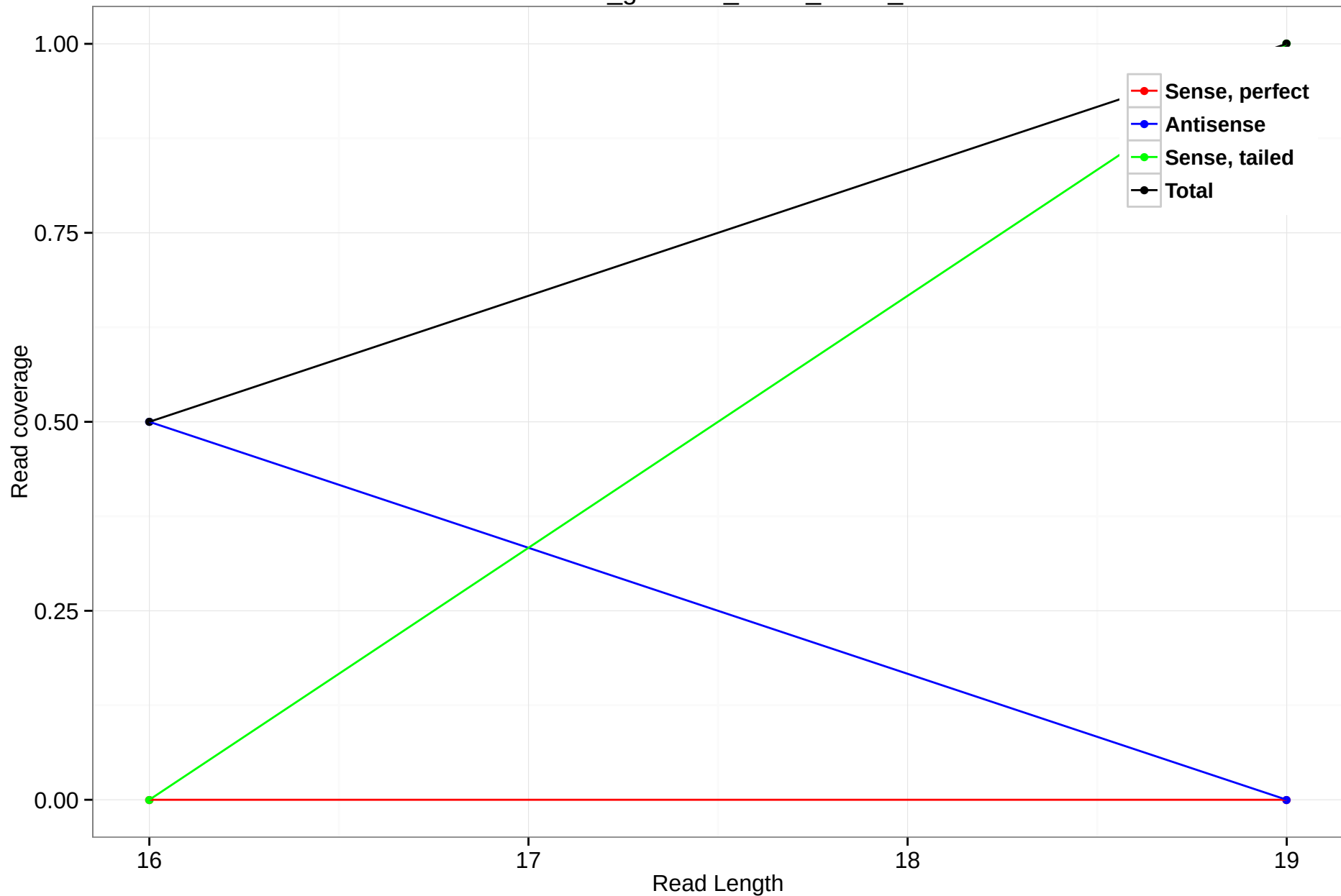
rheMac3_genscan_chr14_24.39_21
