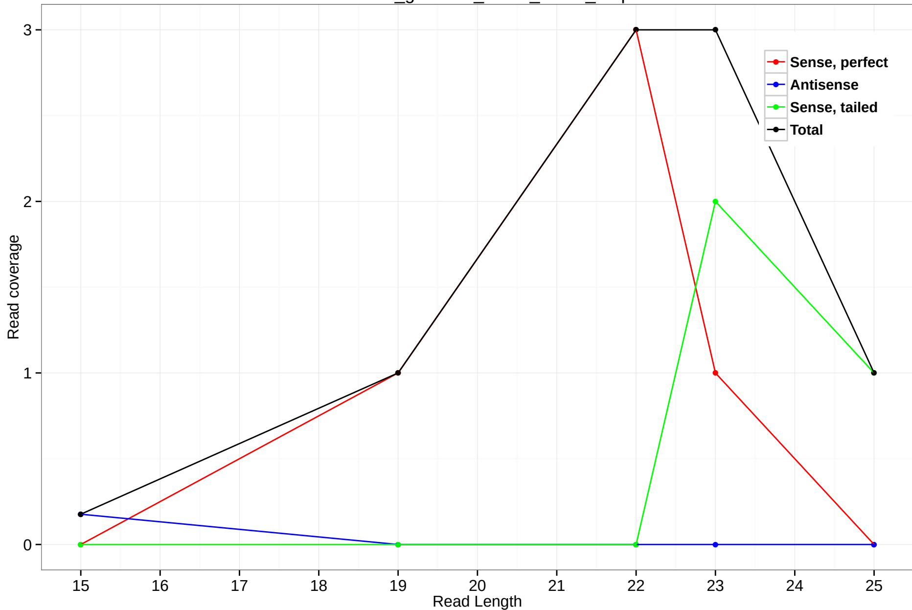
rheMac3_genscan_chr14_24.23_3.3p
