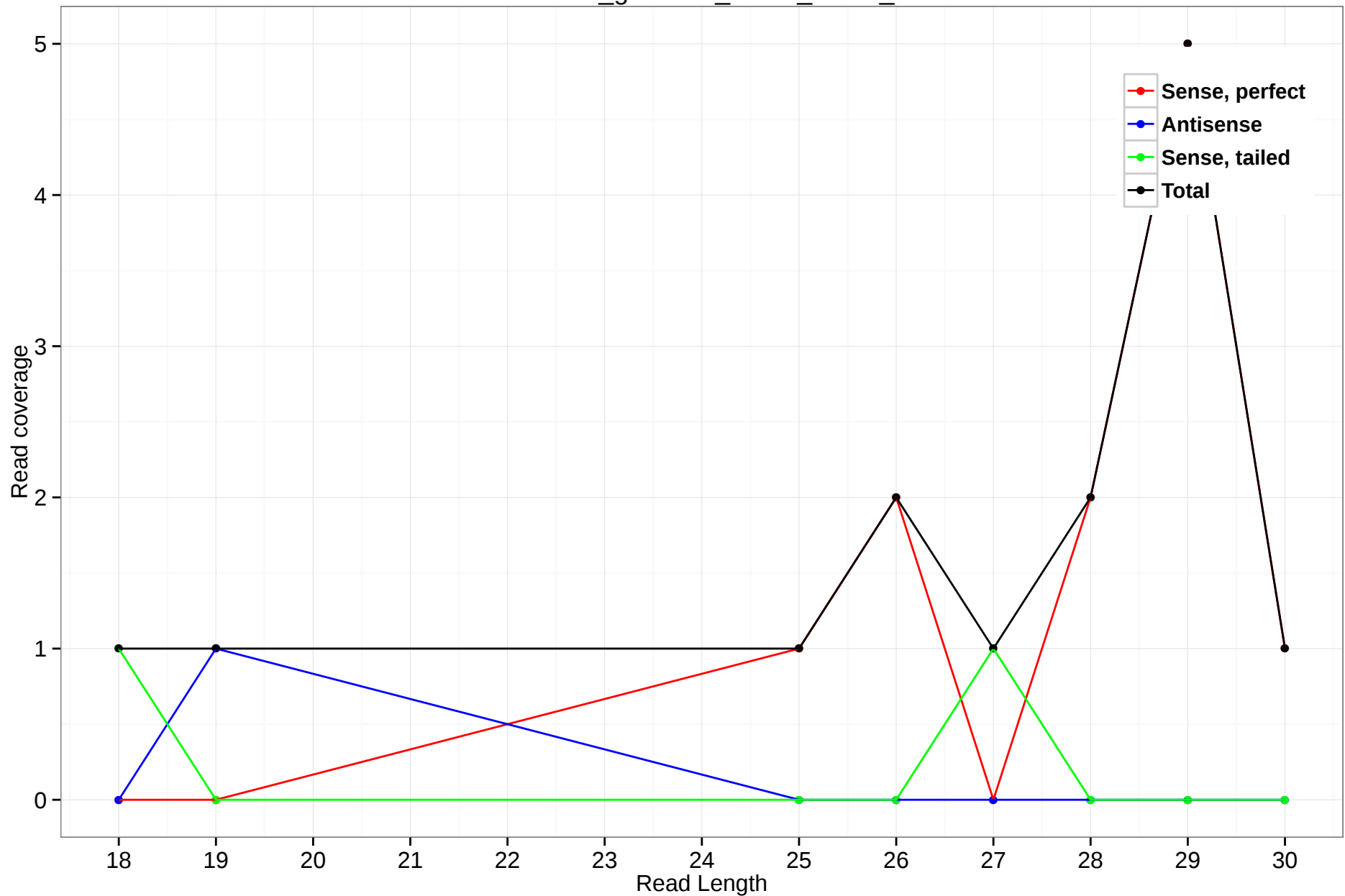
rheMac3_genscan_chr14_24.16_7
