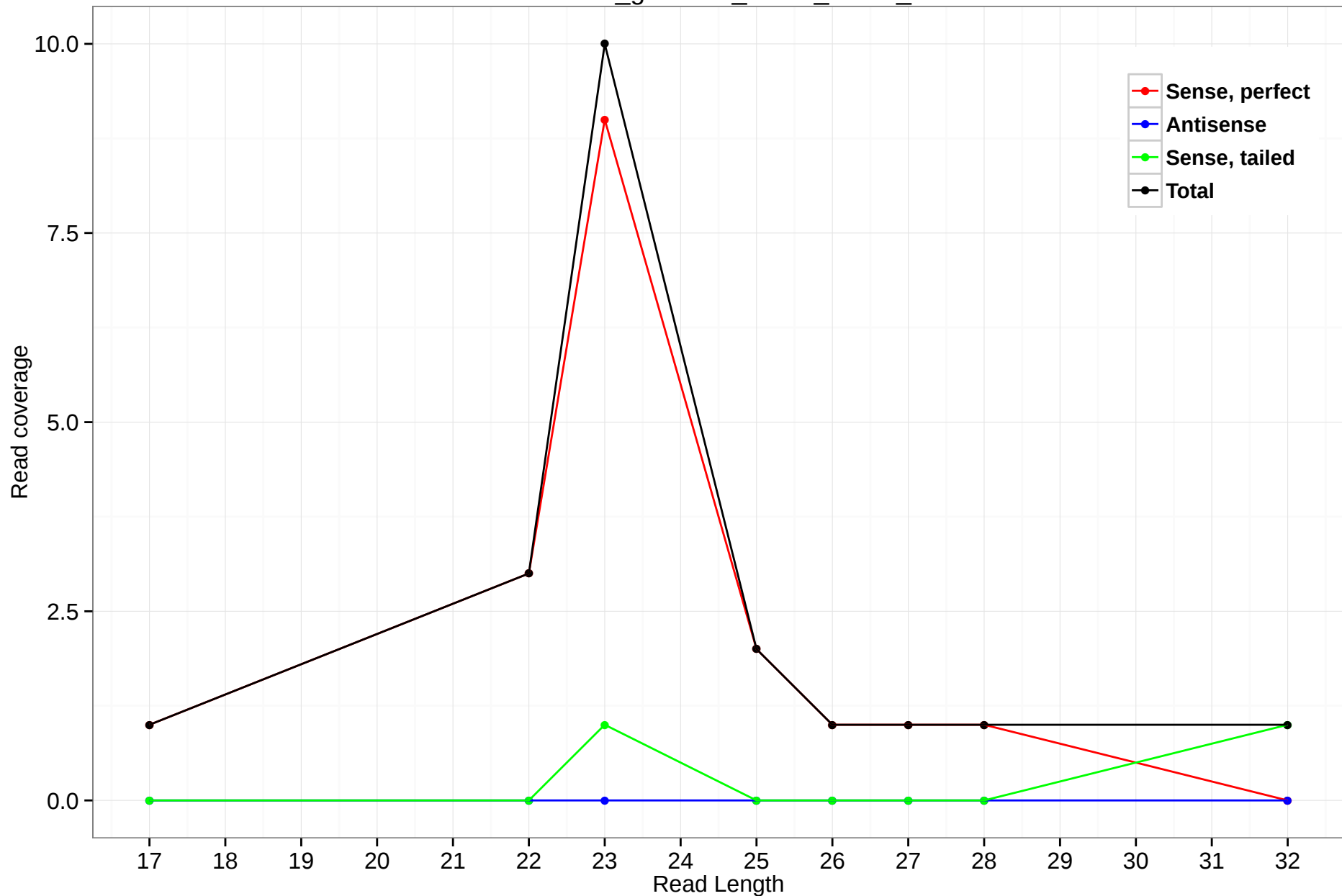
rheMac3_genscan_chr14_16.19_5
